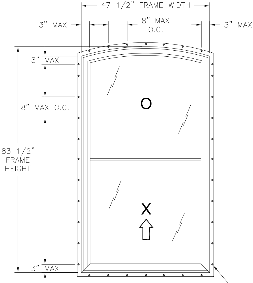
1620/1621 SH REINFORCED DESIGNER EXTERIOR VIEW FIN INSTALLATION
