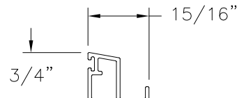
OPERABLE SCREEN TRACK W/O LEG ALUMINUM 6063-T5 (M-2341)
