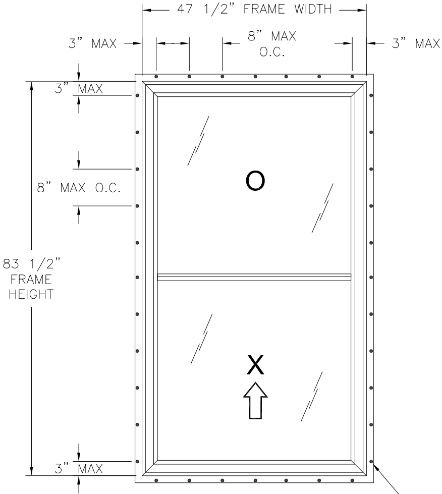
1620/1621 SH REINFORCED RECTANGULAR EXTERIOR VIEW FIN INSTALLATION
