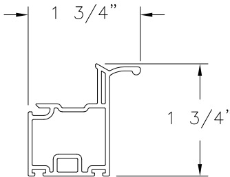
BOTTOM SASH/BOTTOM RAIL EXTRUDED PVC (V-672)
