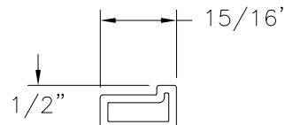
LOCK RAIL REINFORCEMENT ALUMINUM 6063-T5 (M-2115)
