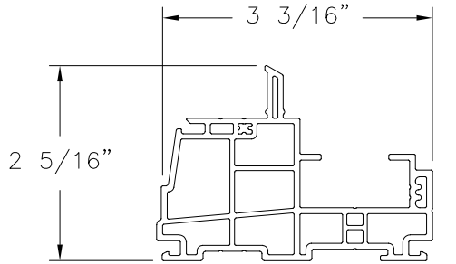
HEAD/JAMB FINLESS EXTRUDED PVC (V-1008)
