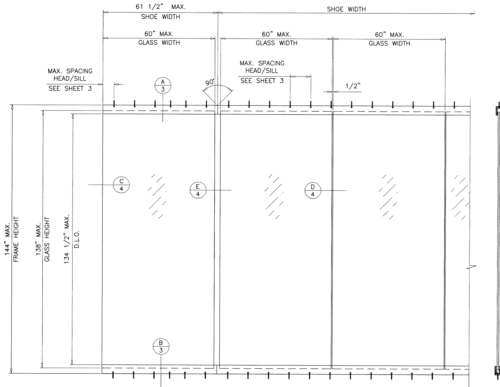
TYPICAL ELEVATION
