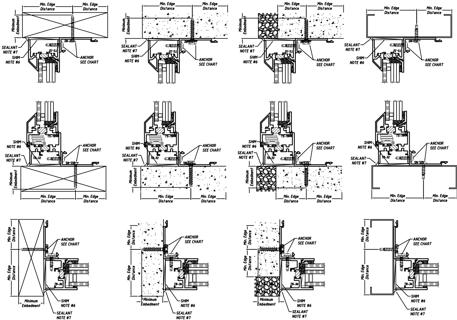
HEAD
