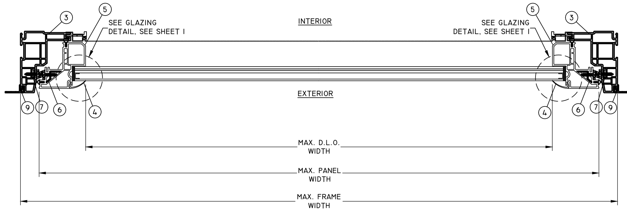
A 4 HORIZONTAL SECTION THROUGH FRAME INSTALLATION
