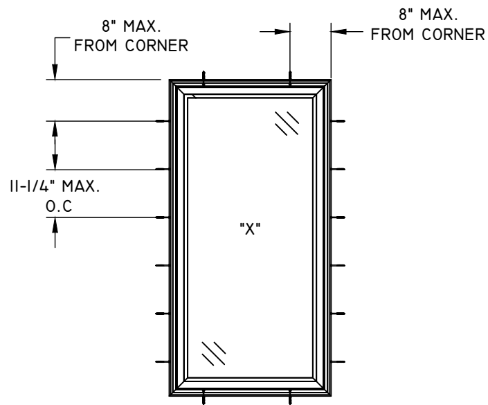
ANCHOR LAYOUT FINLESS
