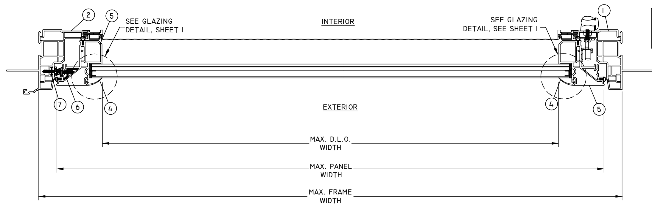
B 4 HORIZONTAL SECTION NAIL FIN INSTALLATION
