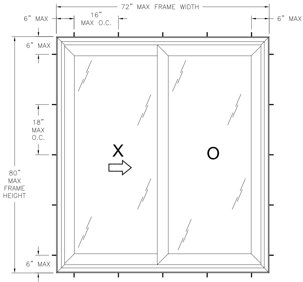
5957 PATIO DOOR OX EXTERIOR VIEW FRAME INSTALLATION
