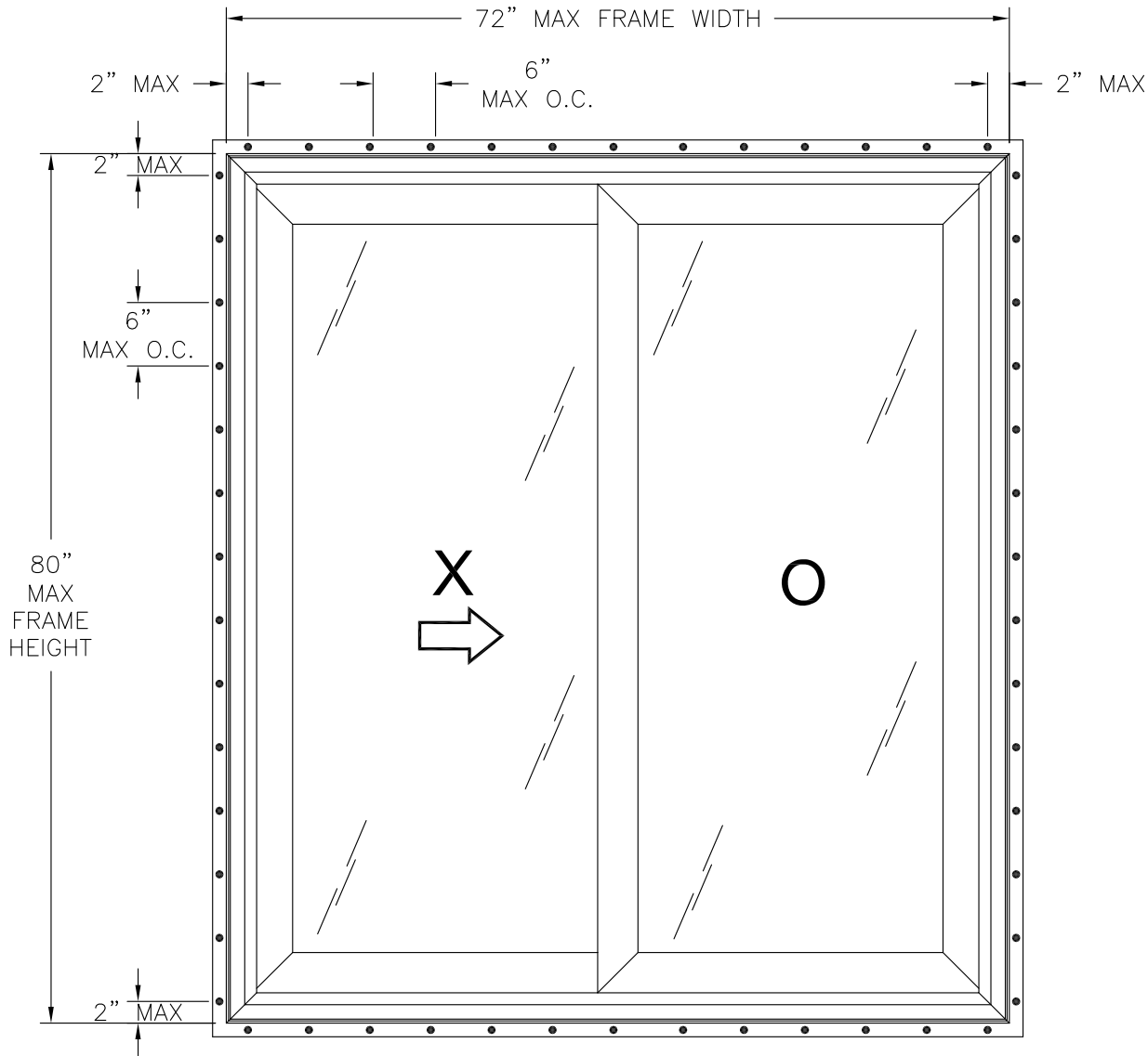
5957 PATIO DOOR OX EXTERIOR VIEW FIN INSTALLATION
