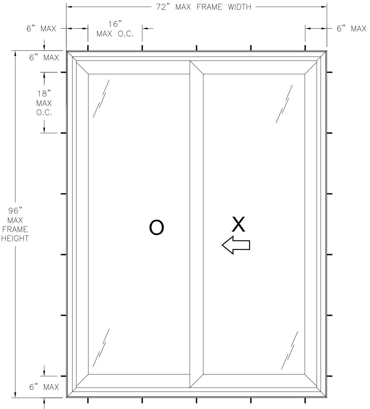
5901/5902 PATIO DOOR OX EXTERIOR VIEW FRAME INSTALLATION
