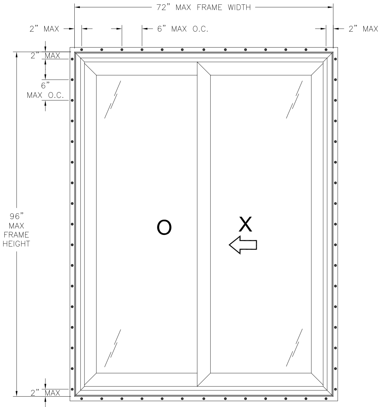
5901/5902 PATIO DOOR OX EXTERIOR VIEW FIN INSTALLATION
