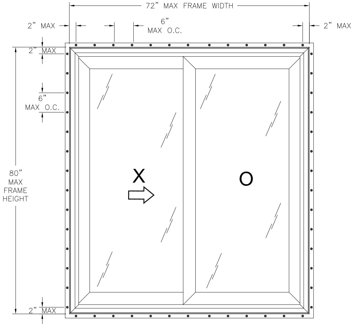
5901/5902 PATIO DOOR OX EXTERIOR VIEW FIN INSTALLATION
