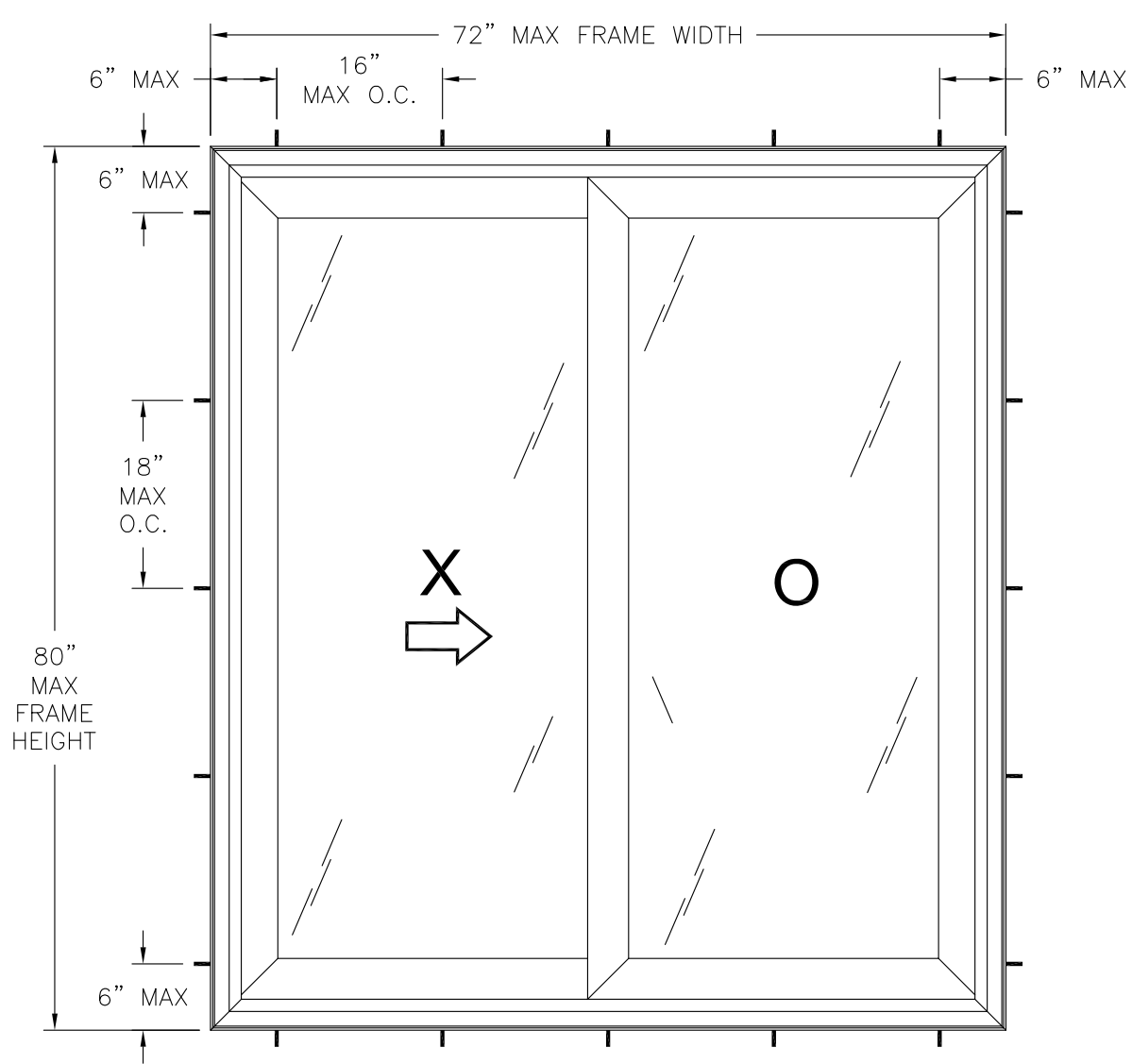
5901/5902 PATIO DOOR OX EXTERIOR VIEW FRAME INSTALLATION
