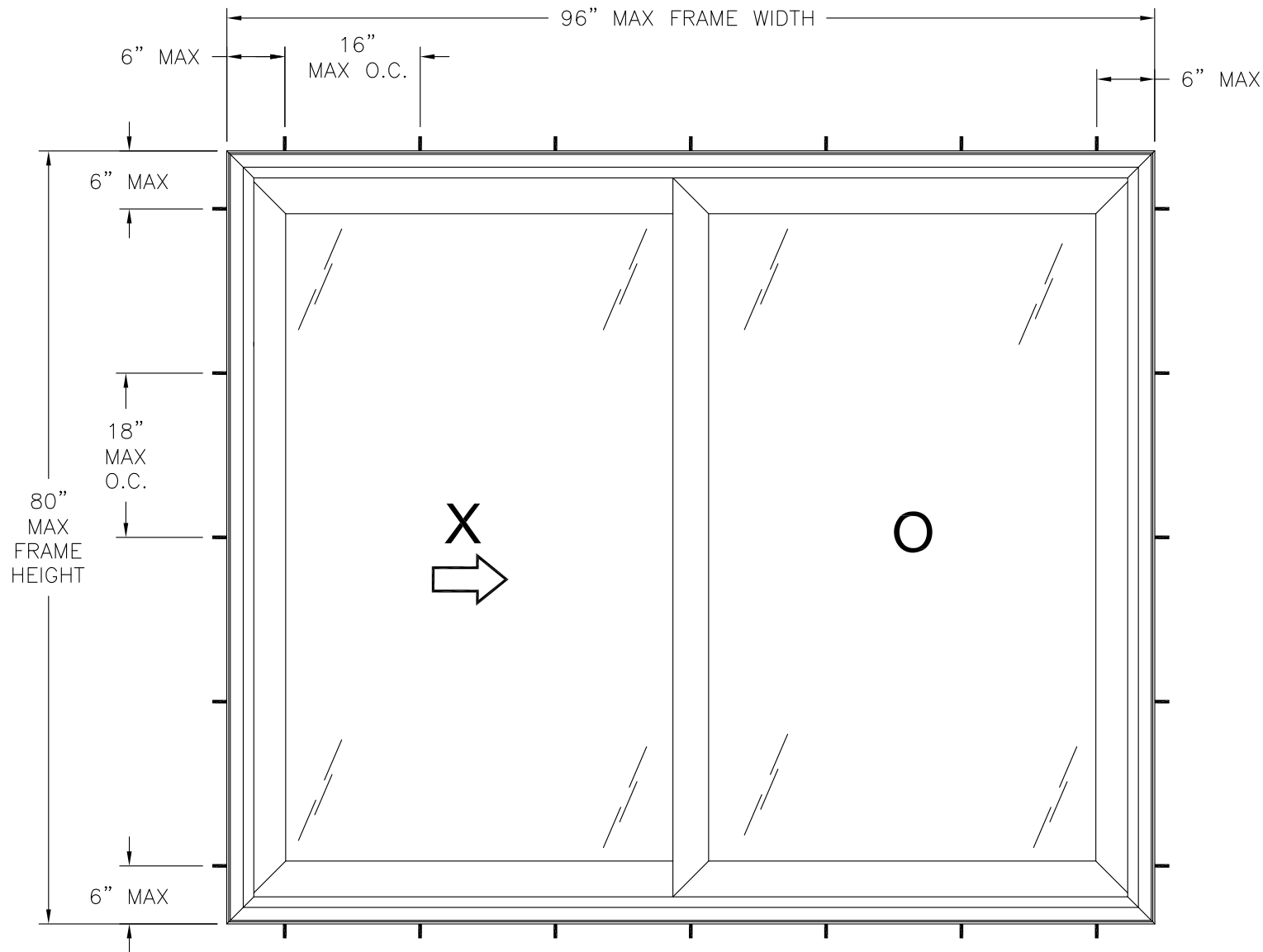
5901/5902 PATIO DOOR OX EXTERIOR VIEW FRAME INSTALLATION
