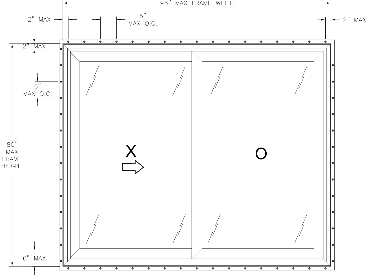
5901/5902 PATIO DOOR OX EXTERIOR VIEW FIN INSTALLATION
