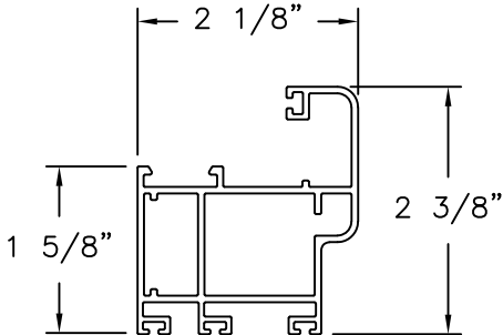
PANEL FRAME ALUMINUM 6063-T6 (MD55006)
