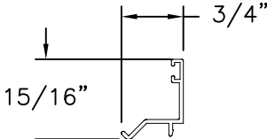
GLASS STOP ALUMINUM 6063-T6 (MD22733)
