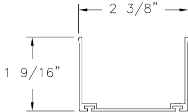
"U" CHANNEL ALUMINUM 6063-T6 (MD45007)
