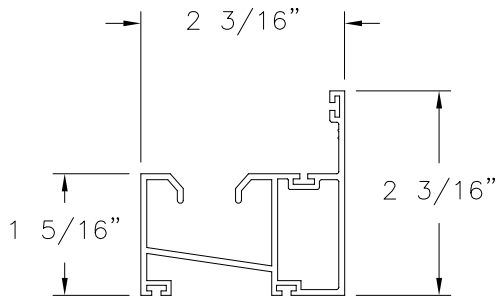
BOTTOM TRACK ALUMINUM 6063-T6 (MD45002)
