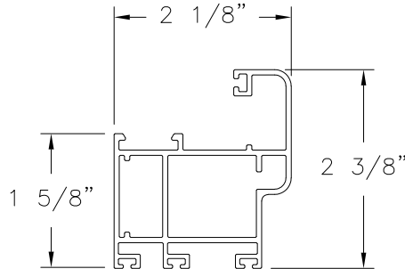
PANEL FRAME ALUMINUM 6063-T6 (MD55006)
