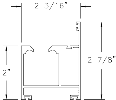
TOP TRACK ALUMINUM 6063-T6 (MD45001)
