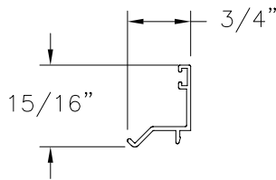
GLASS STOP ALUMINUM 6063-T6 (MD22733)
