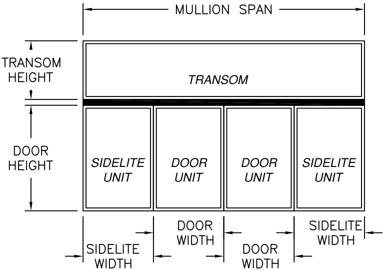
HORIZONTAL MULLION DOUBLE DOOR WITH SIDELITE & TRANSOM SEE CHARTS #74, #75, #76, #77 AND #78 FOR RATINGS
