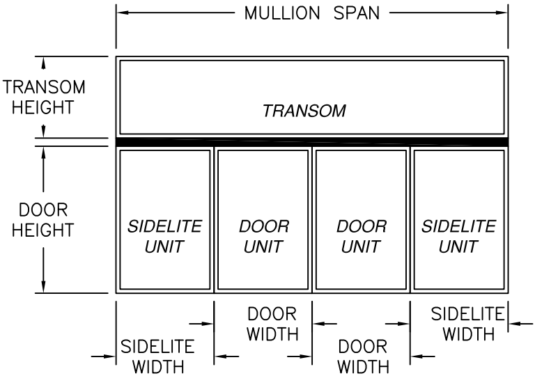
HORIZONTAL MULLION DOUBLE DOOR WITH SIDELITES AND TRANSOM SEE CHARTS #84, #85, #86, AND #88 FOR RATINGS
