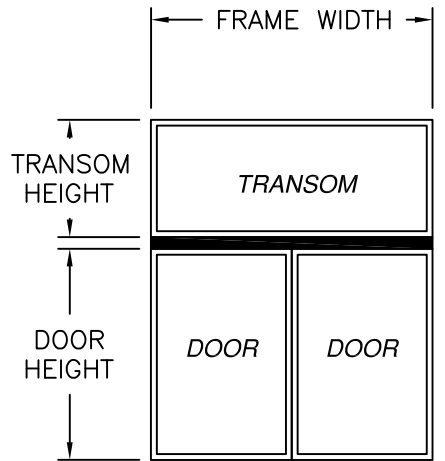
HORIZONTAL MULLION DOUBLE DOOR WITH TRANSOM SEE CHARTS #5, #6, #7, AND #8 FOR RATINGS
