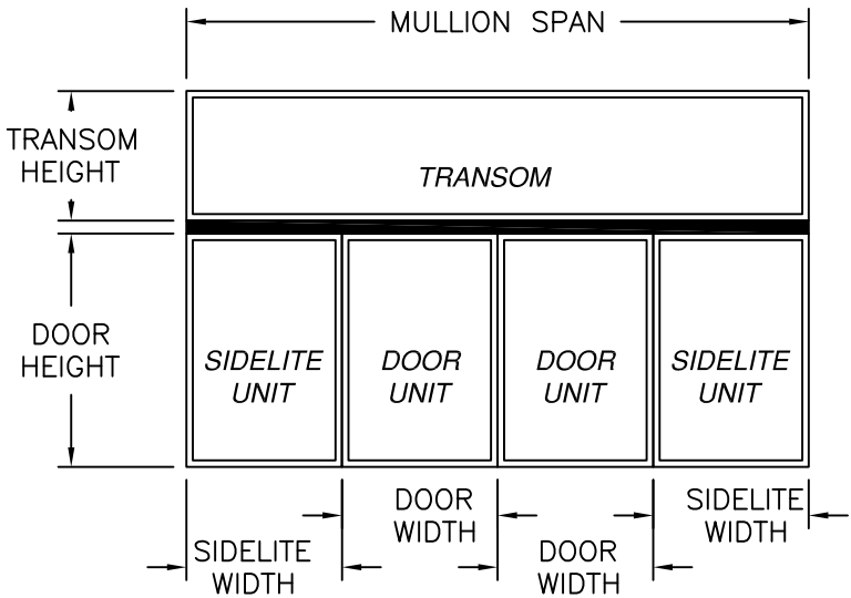
HORIZONTAL MULLION DOUBLE DOOR WITH SIDELITES & TRANSOM SEE CHARTS #69, #70, #71, #72 AND #73 FOR RATINGS
