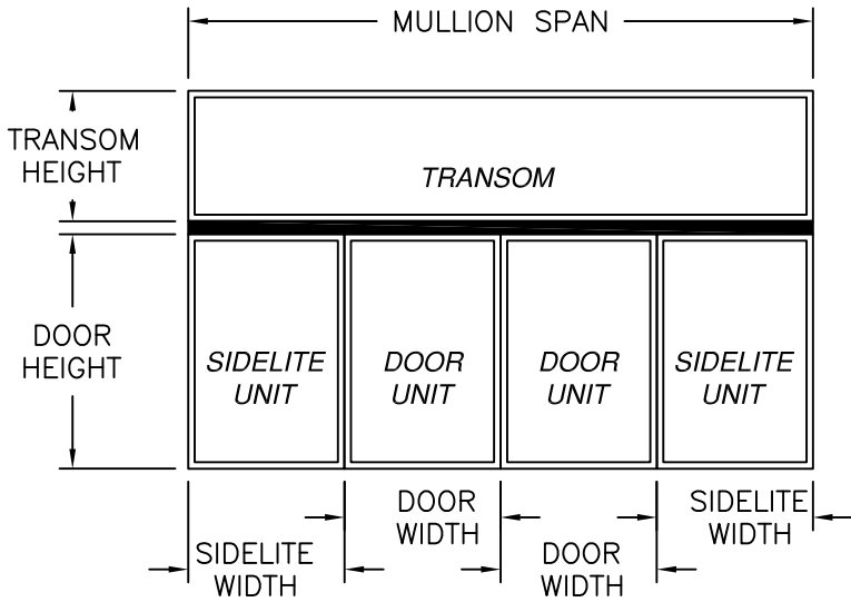
HORIZONTAL MULLION DOUBLE DOOR WITH SIDELITES AND TRANSOM SEE CHARTS #79, #80, #81, #82 AND #83 FOR RATINGS
