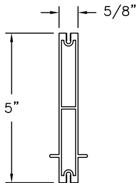
MULLION ALUMINUM 6063-T5 .079" THICK
