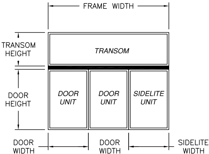
HORIZONTAL MULLION DOUBLE DOOR WITH SIDELITE & TRANSOM SEE CHARTS #59, #60, #61, #62 AND #63 FOR RATINGS
