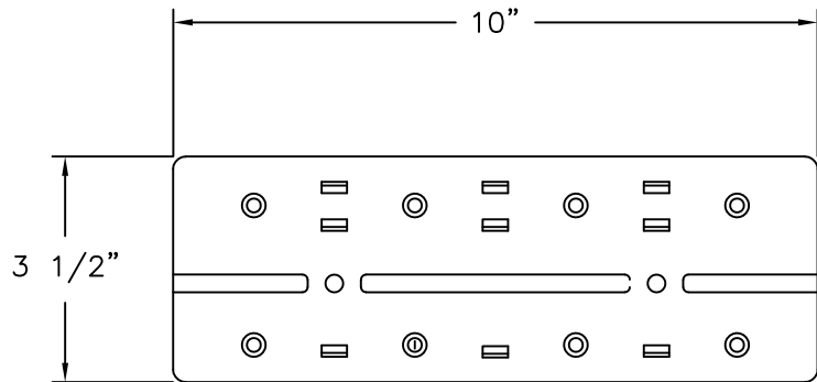
CONNECTION PLATE STAINLESS STEEL .060" THICK
