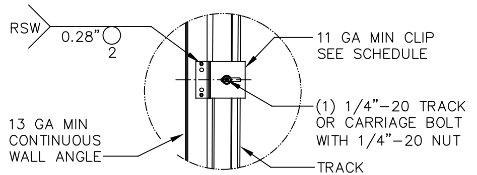
TYPICAL CLIP WELDING DETAIL
