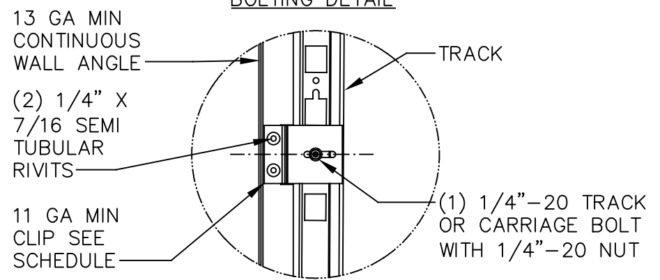
TYPICAL CLIP RIVETING DETAIL
