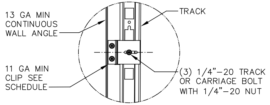
TYPICAL CLIP BOLTING DETAIL
