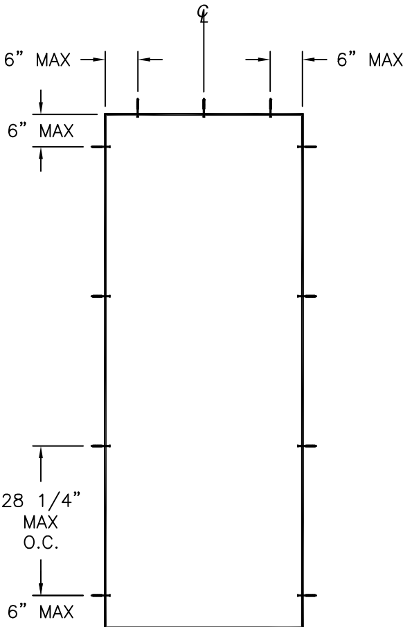
SINGLE DOOR ANCHORING LAYOUT FRAME INSTALLATION
