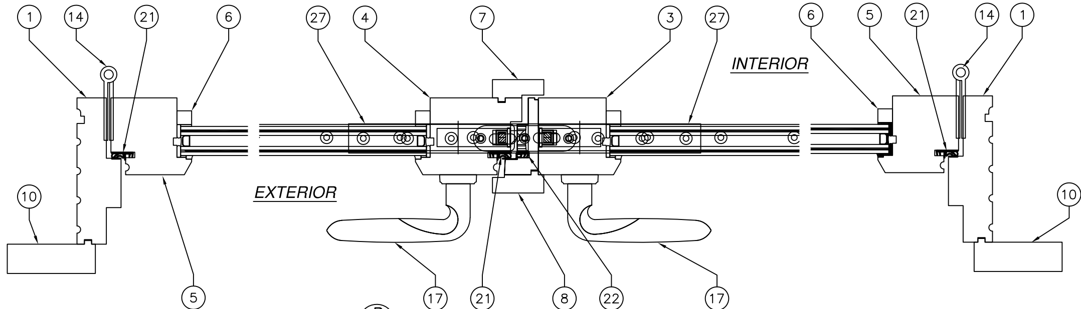
D 8 HORIZONTAL SECTION
