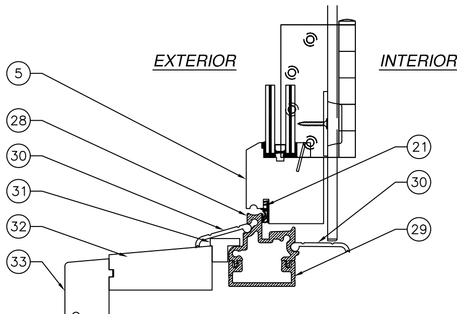
C 8 VERTICAL SECTION WITH BRONZE SILL
