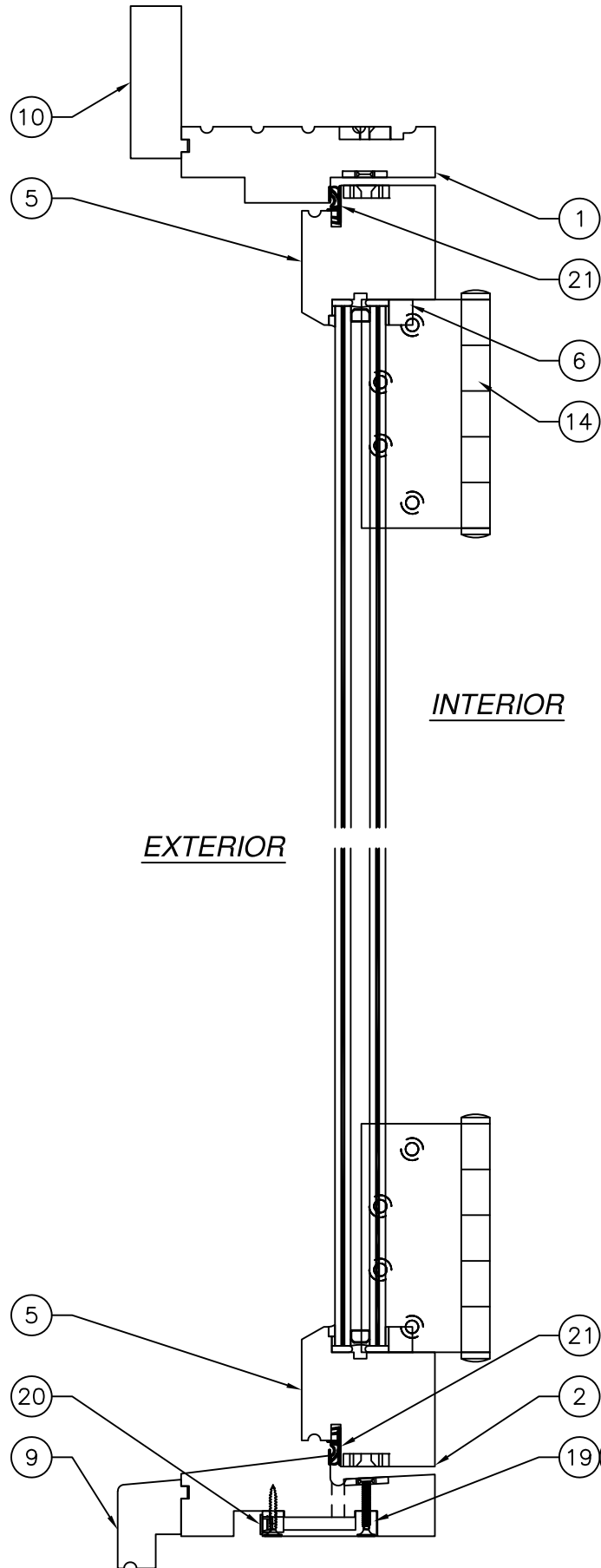
C 8 VERTICAL SECTION WITH WOOD SILL
