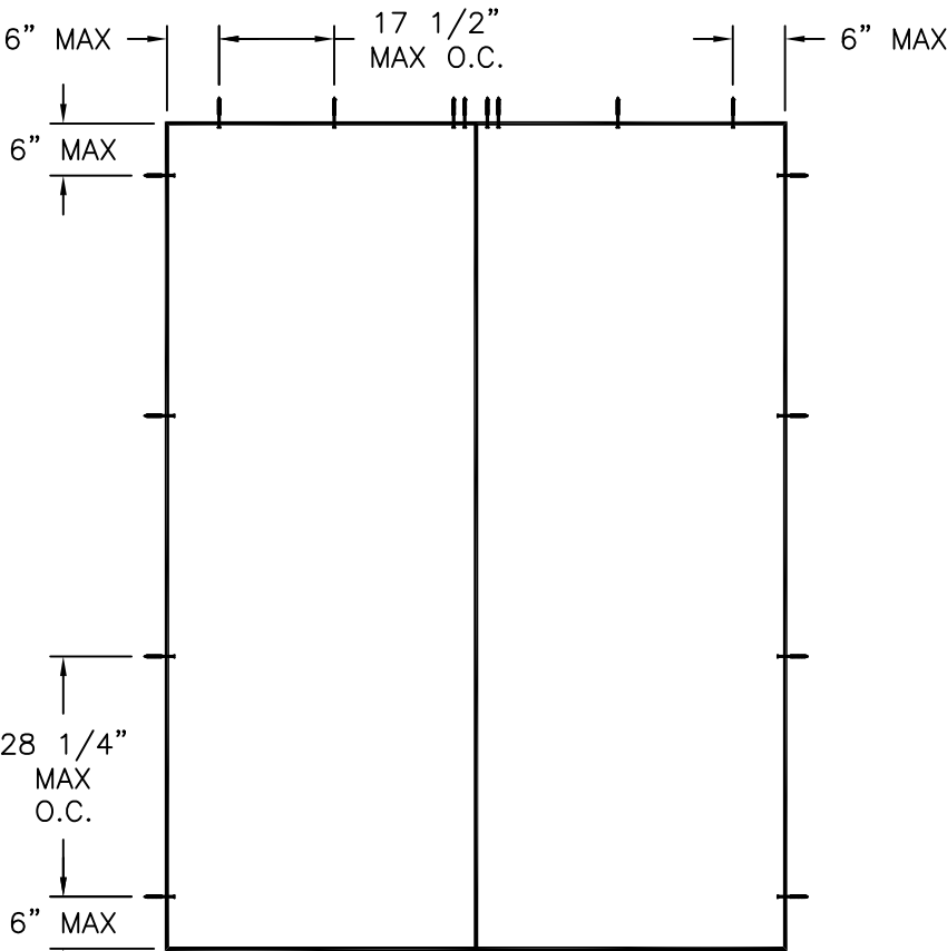
DOUBLE DOOR ANCHORING LAYOUT FRAME INSTALLATION
