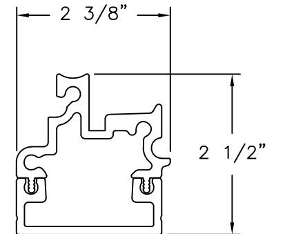
SILL ALUMINUM 6063-T5 .125" THICK
