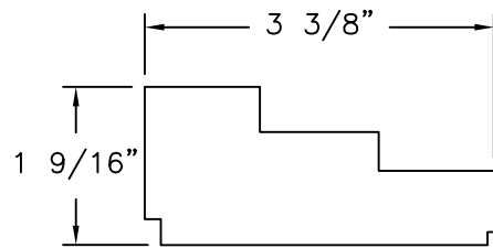
INACTIVE ASTRAGAL (AS3.3) MAHOGANY
