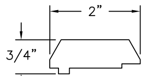
EXTERIOR ASTRAGAL (AS2) MAHOGANY
