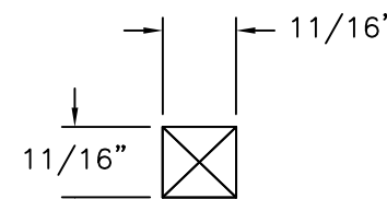
GLASS STOP BLOCK (BL1) MAHOGANY
