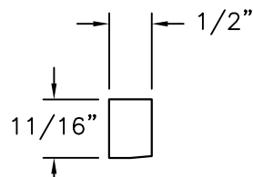
GLASS STOP (GSA) MAHOGANY
