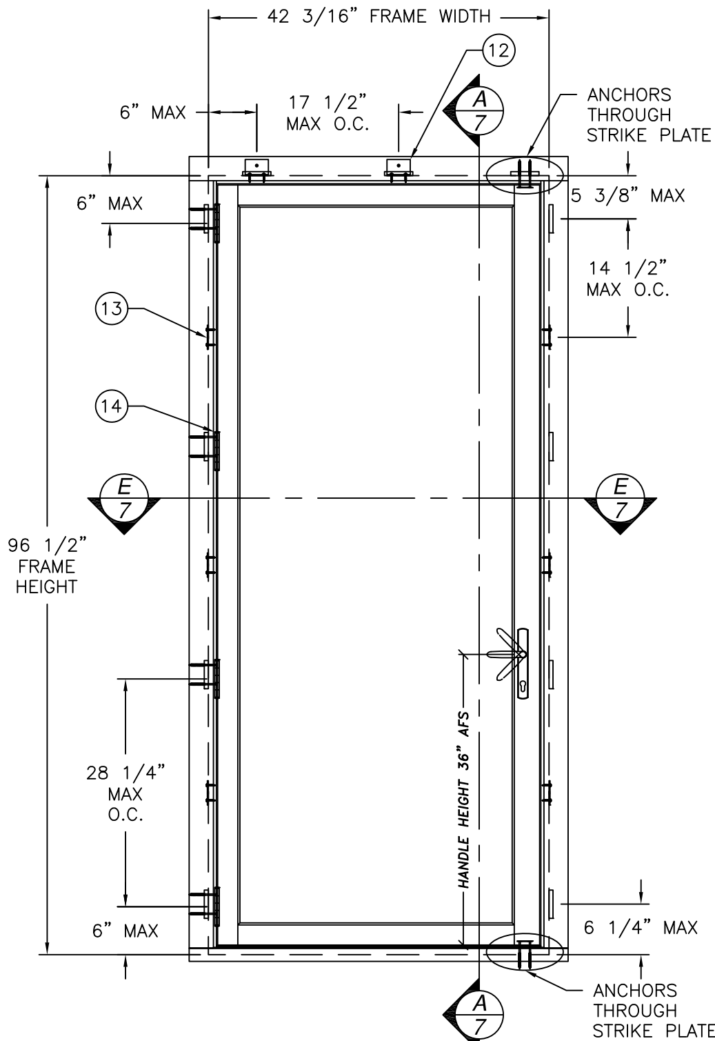
RWD WOOD FRENCH OUT-SWING SINGLE DOOR EXTERIOR VIEW WITH SINGLE POINT ACCURATE LOCKING SYSTEM
