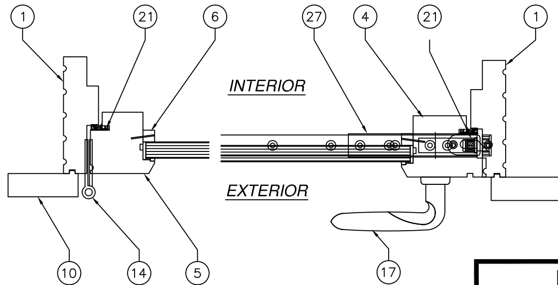
\frac{F}{8} HORIZONTAL SECTION
