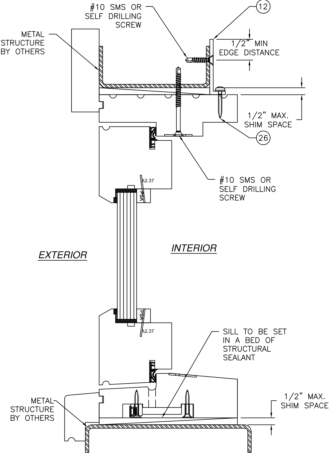
VERTICAL CROSS SECTION METAL STRUCTURE INSTALLATION STANDARD SILL SHOWN, SEE SHEET 20 FOR BRONZE SILL INSTALLATION
