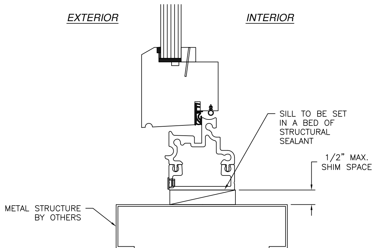
VERTICAL CROSS SECTION METAL STRUCTURE INSTALLATION
