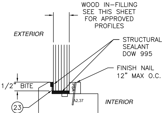
IN-FILLING DETAIL
