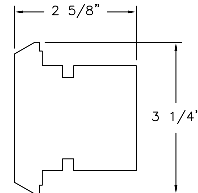
⑳ LOCK RAIL MAHOGANY
