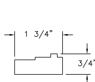
⑦ ASTRAGAL WOOD MAHOGANY
