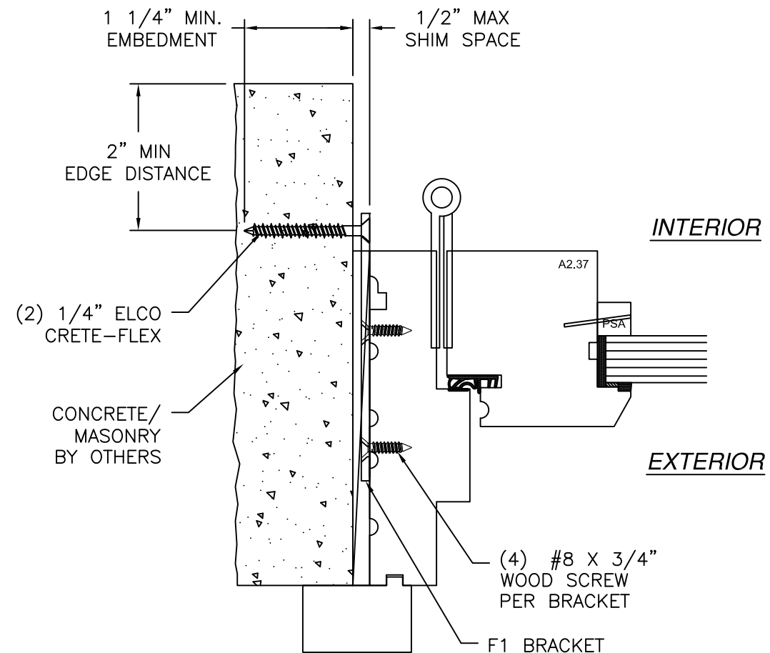
HORIZONTAL CROSS SECTION CONCRETE/MASONRY WITHOUT 1X BUCK INSTALLATION FOR CONCRETE/MASONRY WITH 1X BUCK REFER TO HEAD AND SILL INSTALLATION DETAILS
