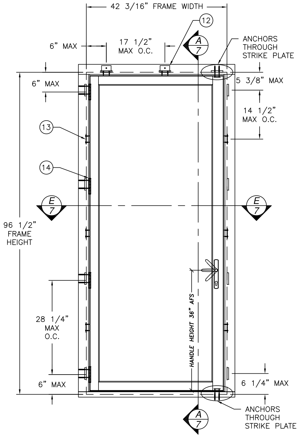
RWD WOOD FRENCH IN-SWING SINGLE DOOR EXTERIOR VIEW WITH SINGLE POINT HOPPE LOCKING SYSTEM
