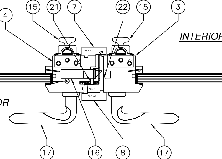
B 7 HORIZONTAL SECTION
