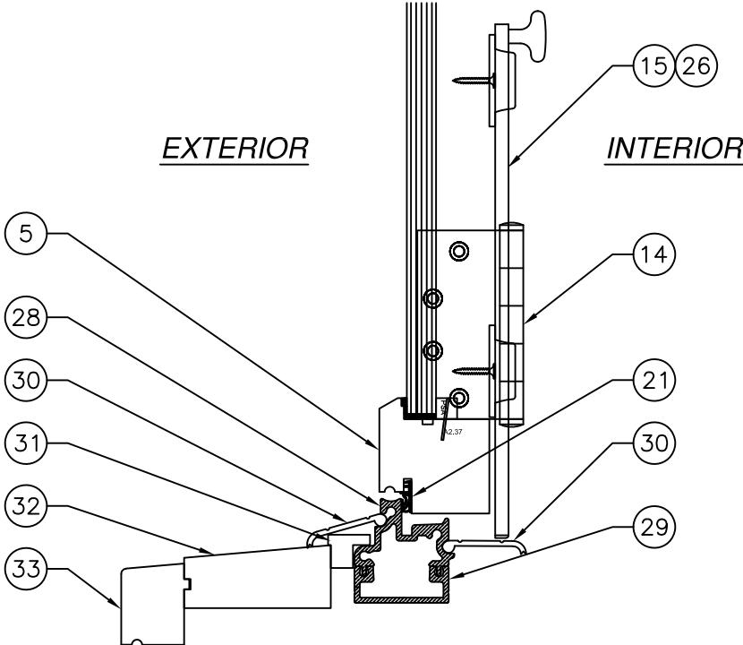
A 7 VERTICAL SECTION WITH BRONZE SILL
