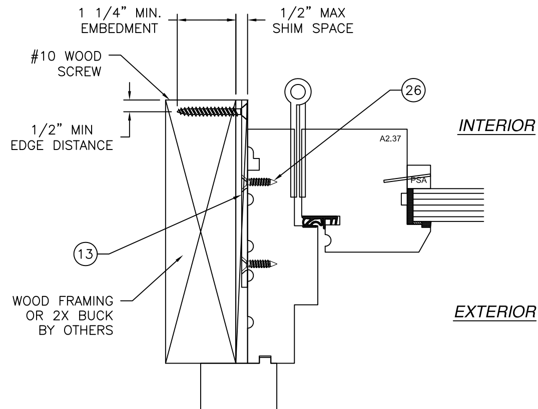
HORIZONTAL CROSS SECTION WOOD FRAMING OR 2X BUCK INSTALLATION
