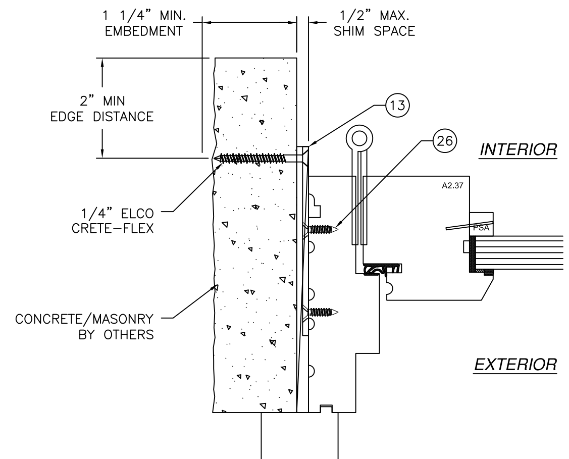
HORIZONTAL CROSS SECTION CONCRETE/MASONRY WITHOUT 1X BUCK INSTALLATION FOR CONCRETE/MASONRY WITH 1X BUCK REFER TO HEAD AND SILL INSTALLATION DETAILS
