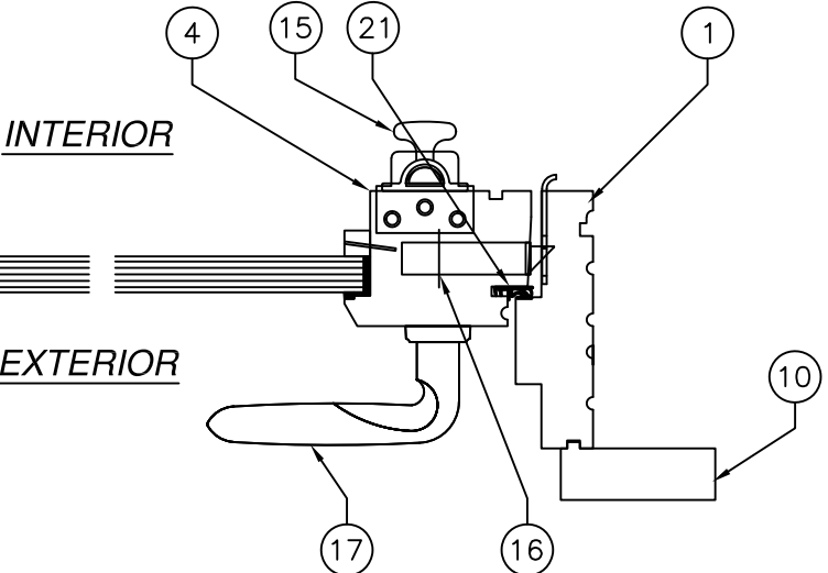
E 7 HORIZONTAL SECTION
