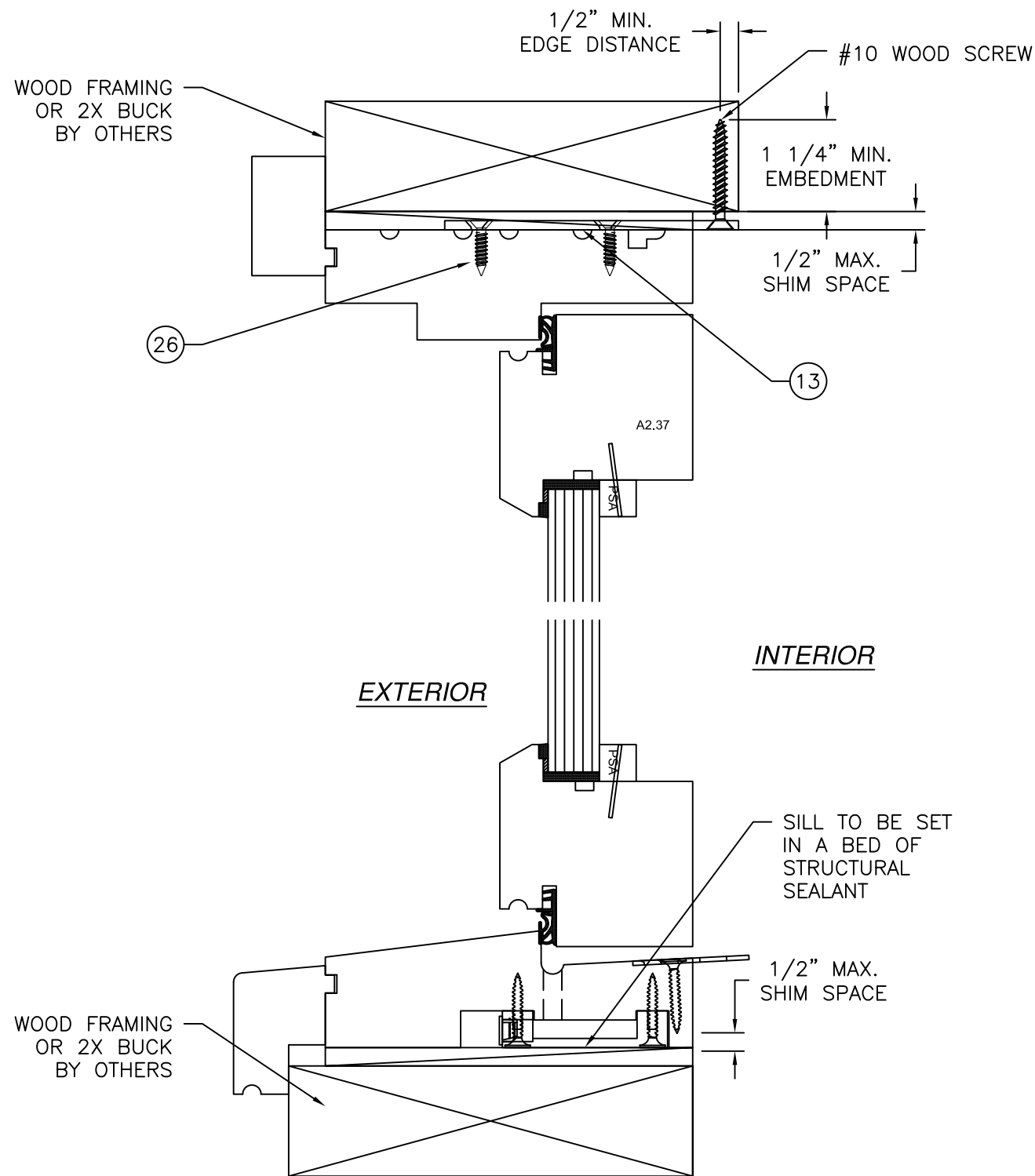
VERTICAL CROSS SECTION WOOD FRAMING OR 2X BUCK INSTALLATION WOOD SILL SHOWN, FOR BRONZE SILL INSTALLATION SEE SHEETS 20 AND 21
