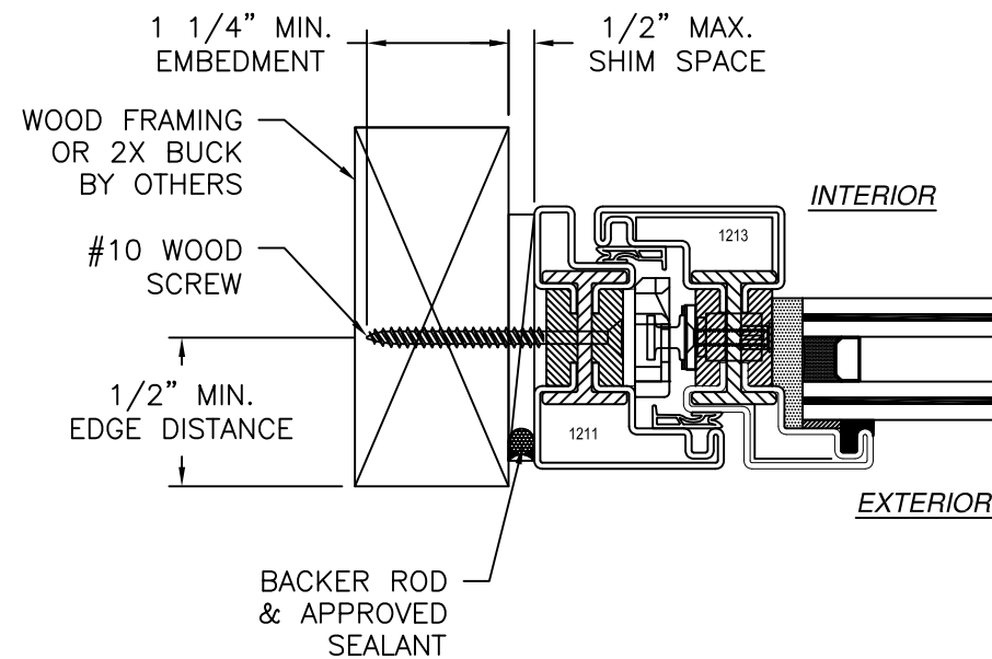
HORIZONTAL CROSS SECTION WOOD FRAMING OR 2X BUCK INSTALLATION
