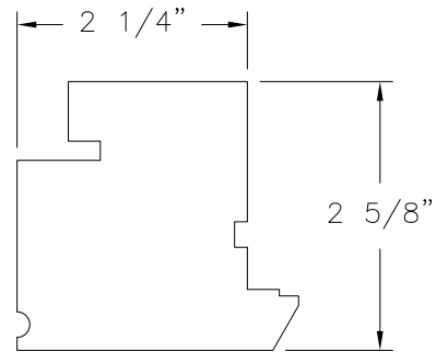
⑤ PANEL FRAME WOOD MAHOGANY
