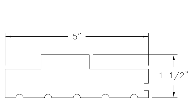
① FRAME WOOD MAHOGANY
