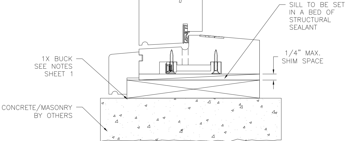
VERTICAL CROSS SECTION CONCRETE/MASONRY INSTALLATION STANDARD SILL SHOWN, SEE SHEET 21 FOR BRONZE SILL INSTALLATION
