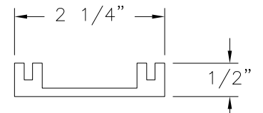
⑪ EXTRUSION ALUMINUM 6063-T5
