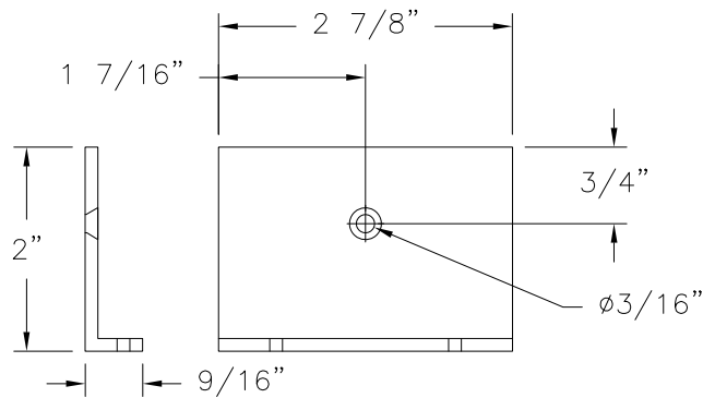
⑫ ANGLE MOUNTING BRACKET ALUMINUM 6063-T5 1/8" THICK
