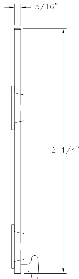
⑮ SURFACE BOLT BRASS
