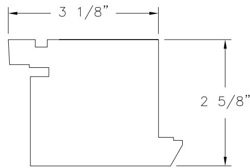
③ STILE WOOD MAHOGANY
