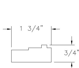
⑧ ⑦ ASTRAGAL WOOD MAHOGANY
