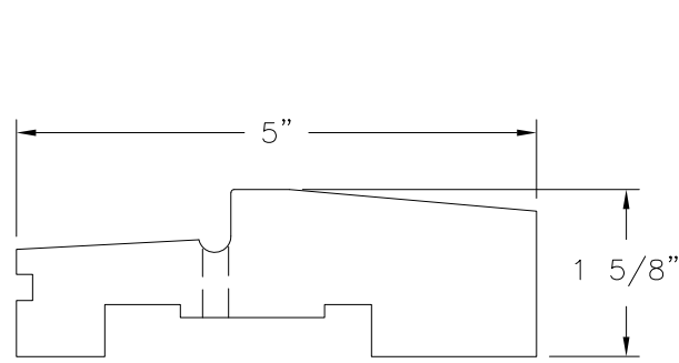
② SILL FRAME WOOD MAHOGANY
