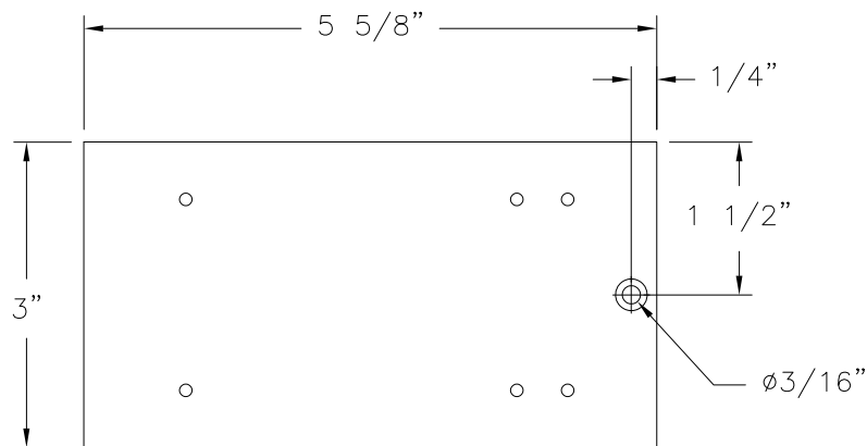
⑫ ANGLE MOUNTING BRACKET ALUMINUM 6063-T5 1/8" THICK
