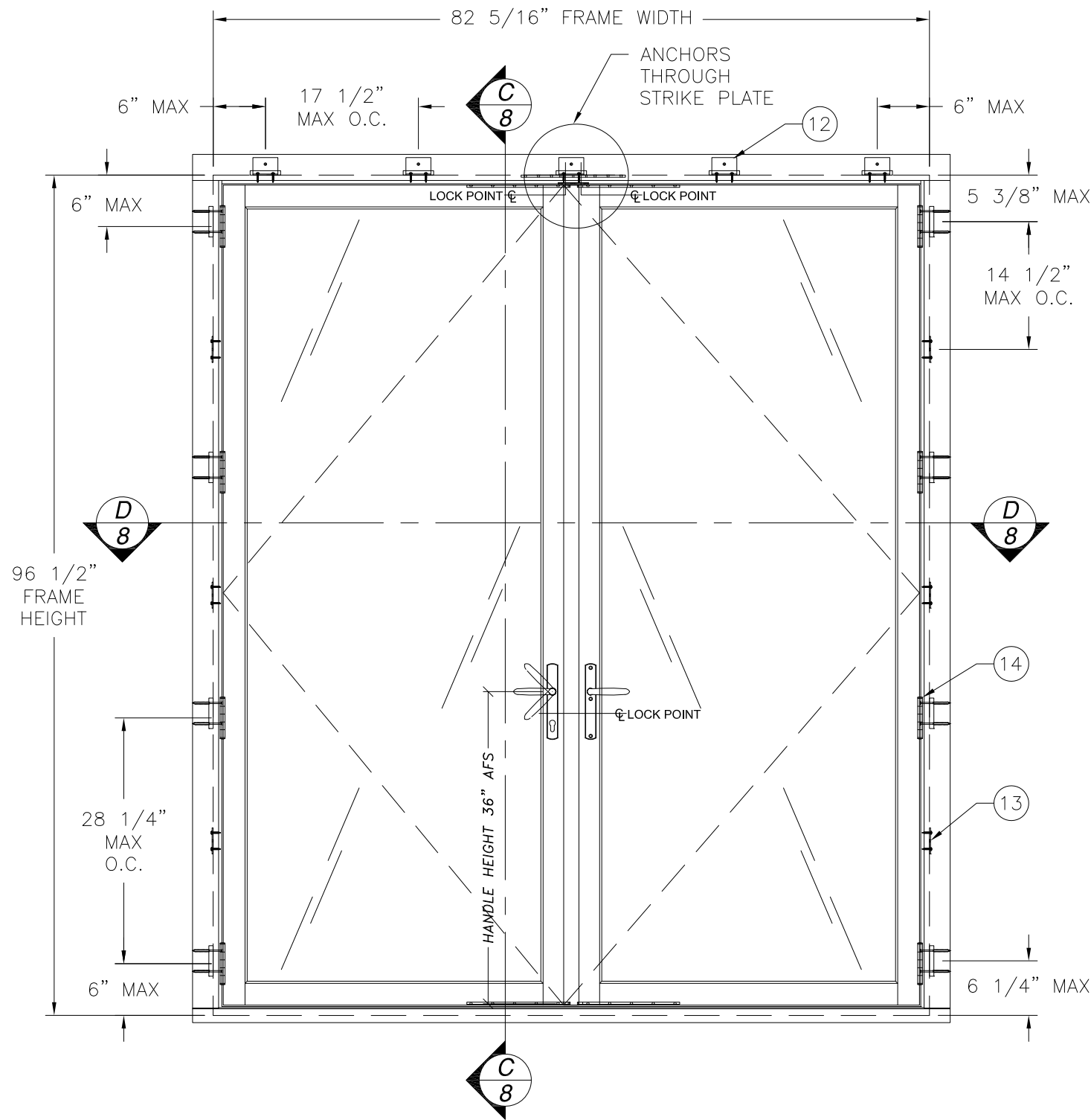
RWD WOOD FRENCH OUT-SWING DOUBLE DOOR EXTERIOR VIEW
