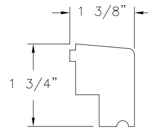
⑨ SILL NOSING WOOD MAHOGANY
