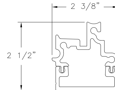
SILL BRONZE
