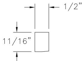
GLASS STOP (GSA) MAHOGANY
