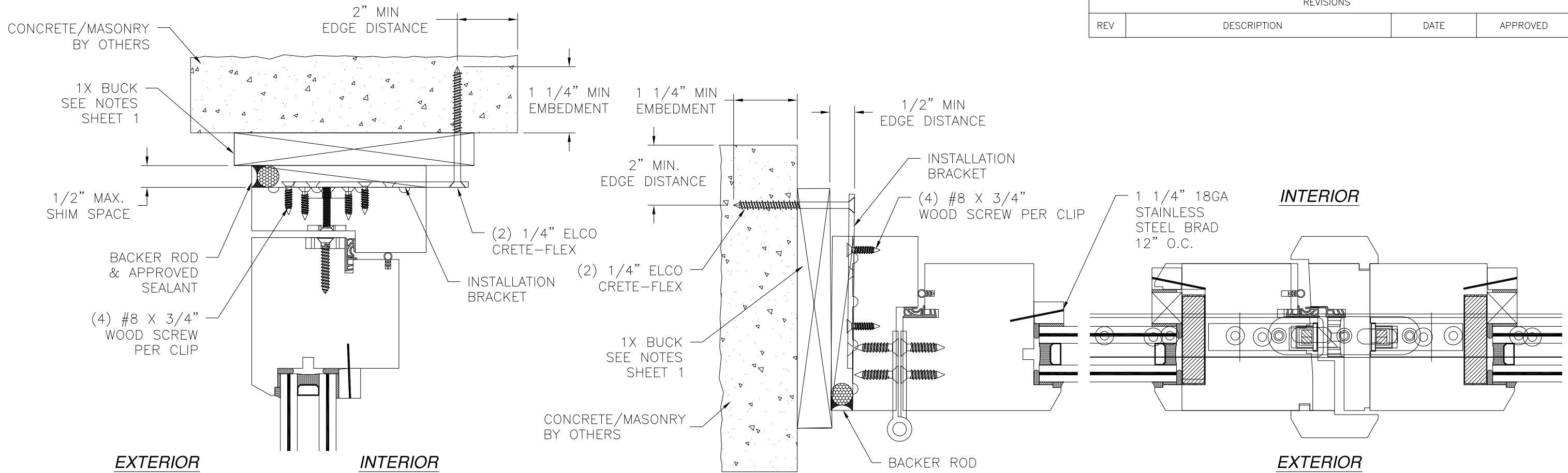
JAMB INSTALLATION DETAIL CONCRETE/MASONRY INSTALLATION
