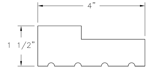
VERTICAL/HORIZONTAL JAMB (J4) MAHOGANY
