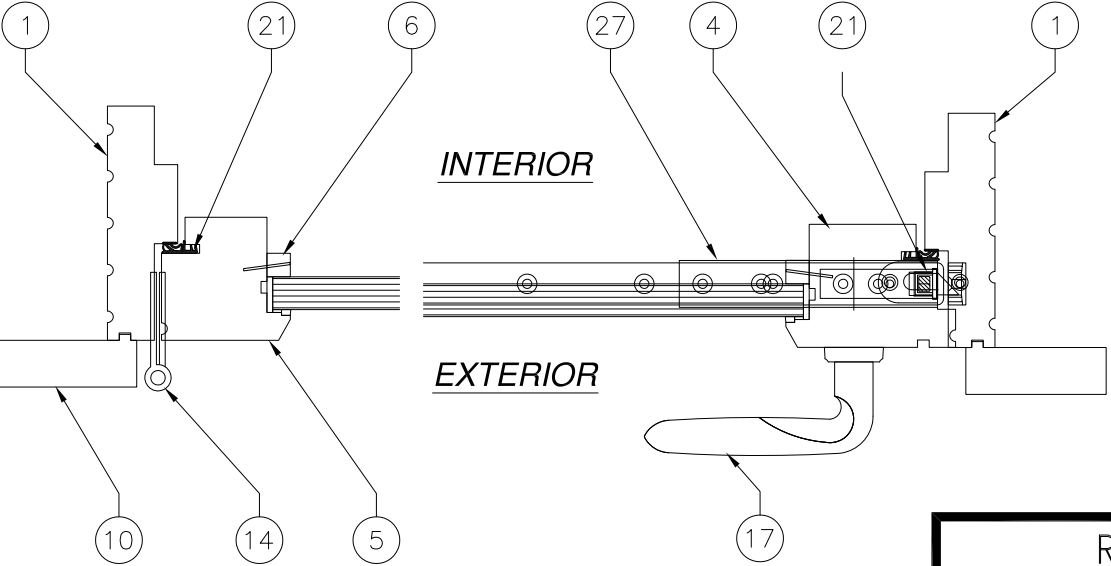
F 8 HORIZONTAL SECTION
