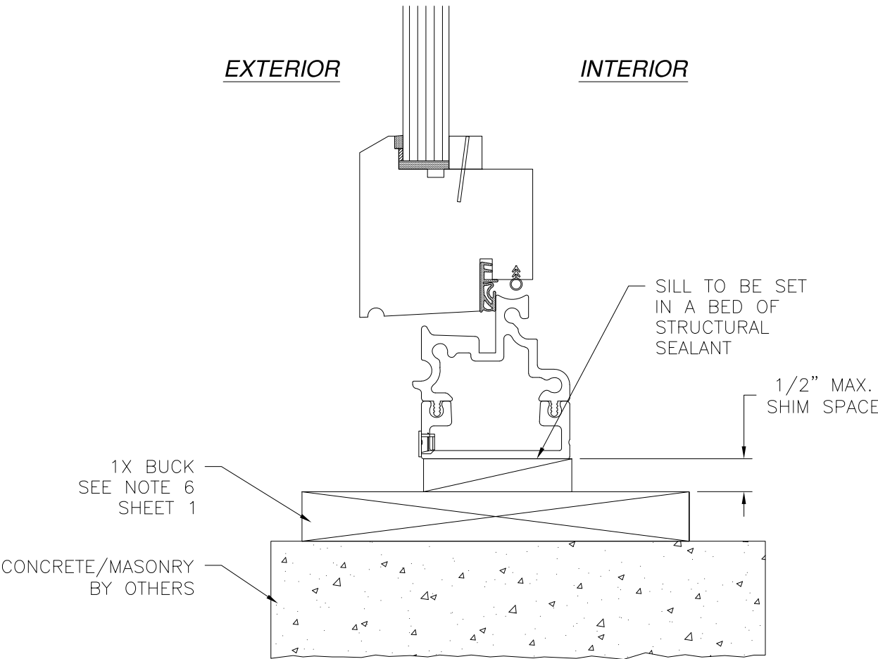
VERTICAL CROSS SECTION CONCRETE/MASONRY WITH 1X BUCK INSTALLATION FOR CONCRETE/MASONRY WITHOUT 1X BUCK REFER TO HORIZONTAL CROSS SECTIONS
