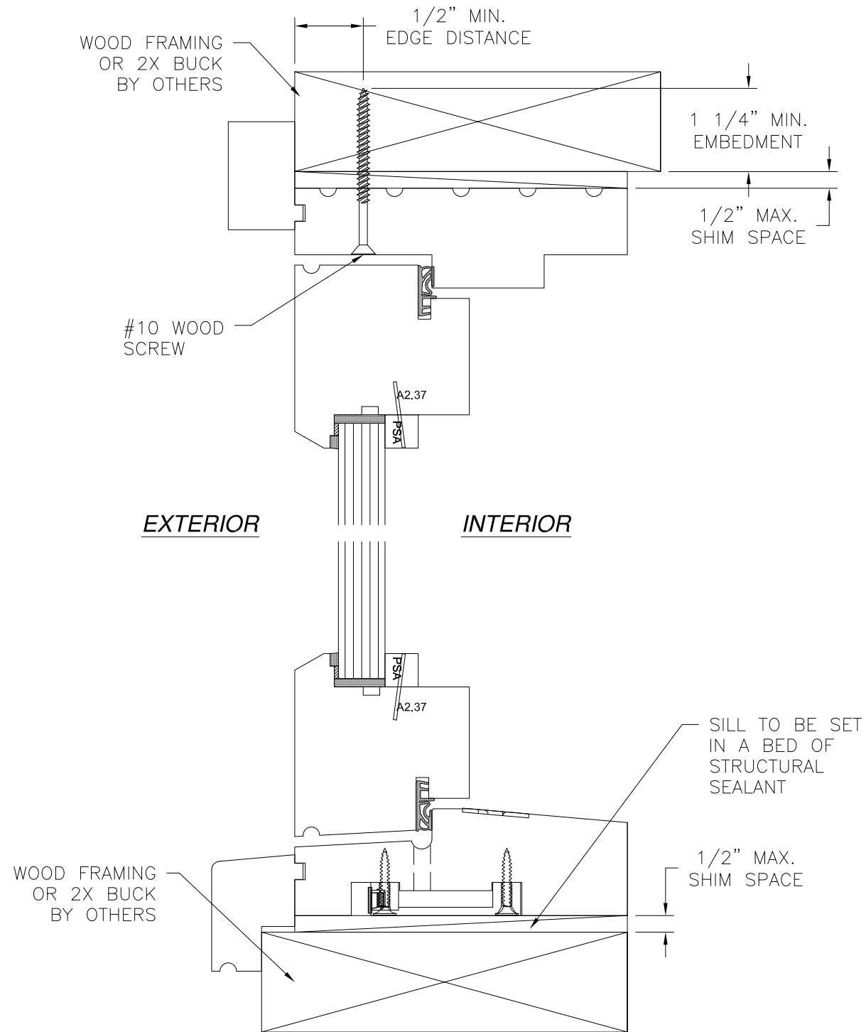
VERTICAL CROSS SECTION WOOD FRAMING OR 2X BUCK INSTALLATION STANDARD SILL SHOWN, SEE SHEET 20 FOR BRONZE SILL INSTALLATION
