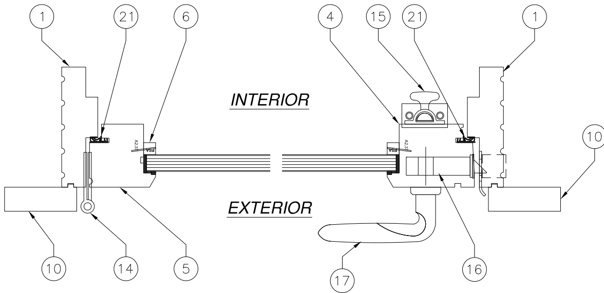
E 7 HORIZONTAL SECTION
