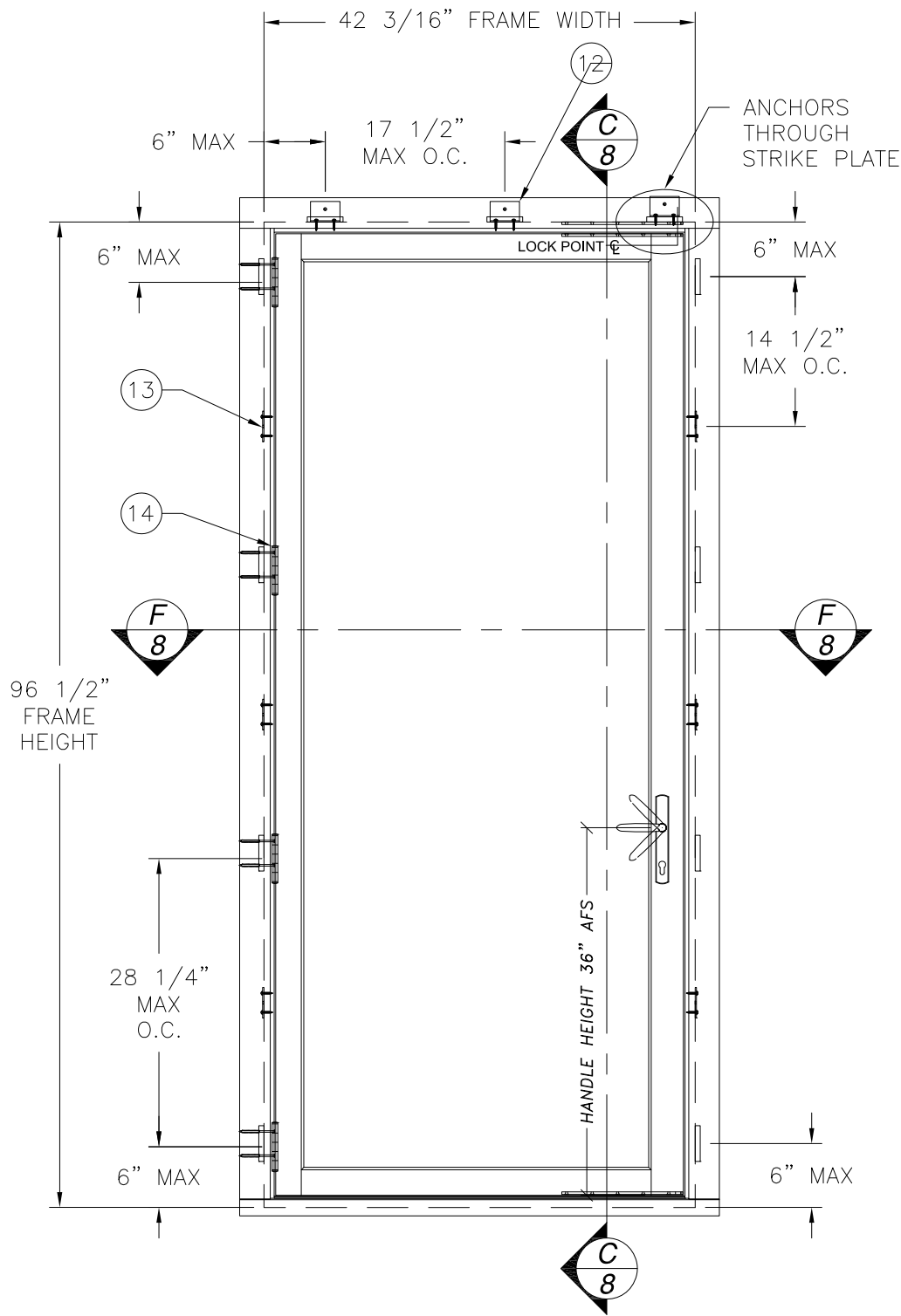
RWD WOOD FRENCH OUT-SWING SINGLE DOOR EXTERIOR VIEW WITH MULTI POINT HOPPE LOCKING SYSTEM
