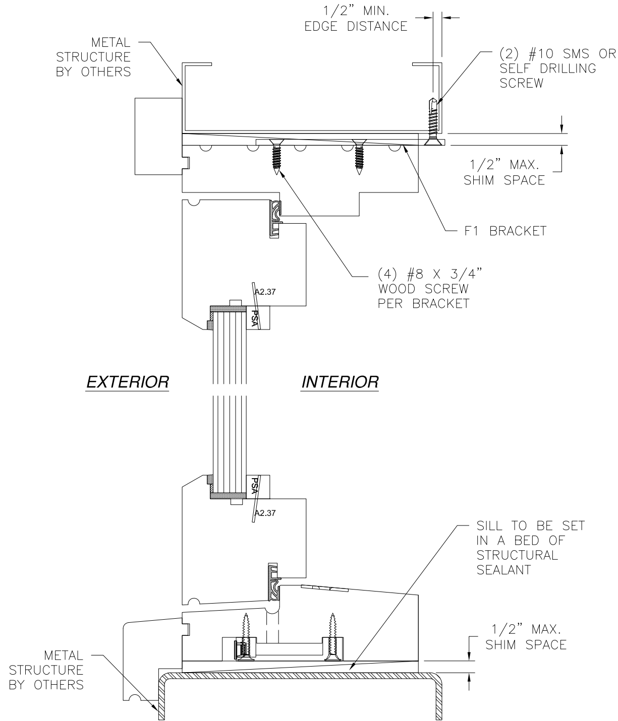
VERTICAL CROSS SECTION METAL STRUCTURE INSTALLATION STANDARD SILL SHOWN, SEE SHEET 20 FOR BRONZE SILL INSTALLATION
