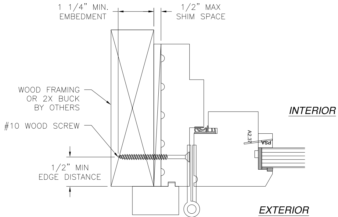
HORIZONTAL CROSS SECTION WOOD FRAMING OR 2X BUCK INSTALLATION
