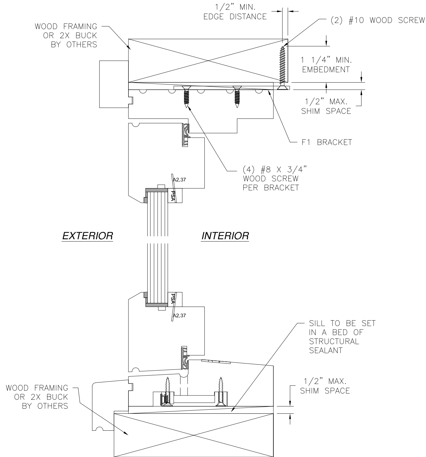
VERTICAL CROSS SECTION WOOD FRAMING OR 2X BUCK INSTALLATION STANDARD SILL SHOWN, SEE SHEET 20 FOR BRONZE SILL INSTALLATION
