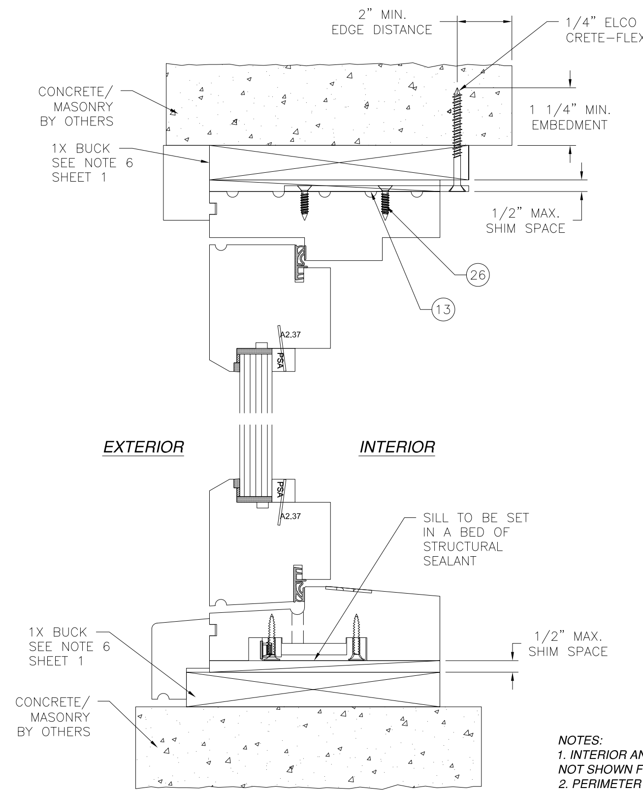
VERTICAL CROSS SECTION CONCRETE/MASONRY WITH 1X BUCK INSTALLATION FOR CONCRETE/MASONRY WITHOUT 1X BUCK REFER TO HORIZONTAL CROSS SECTION STANDARD SILL SHOWN, SEE SHEET 20 FOR BRONZE SILL INSTALLATION
