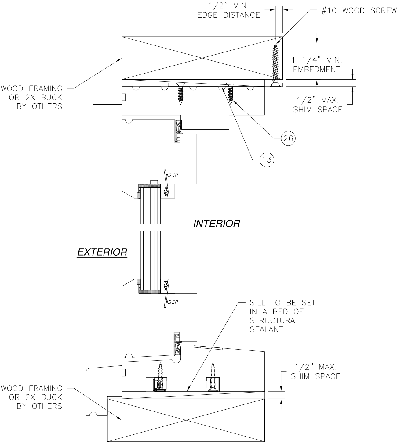
VERTICAL CROSS SECTION WOOD FRAMING OR 2X BUCK INSTALLATION STANDARD SILL SHOWN, SEE SHEET 20 FOR BRONZE SILL INSTALLATION
