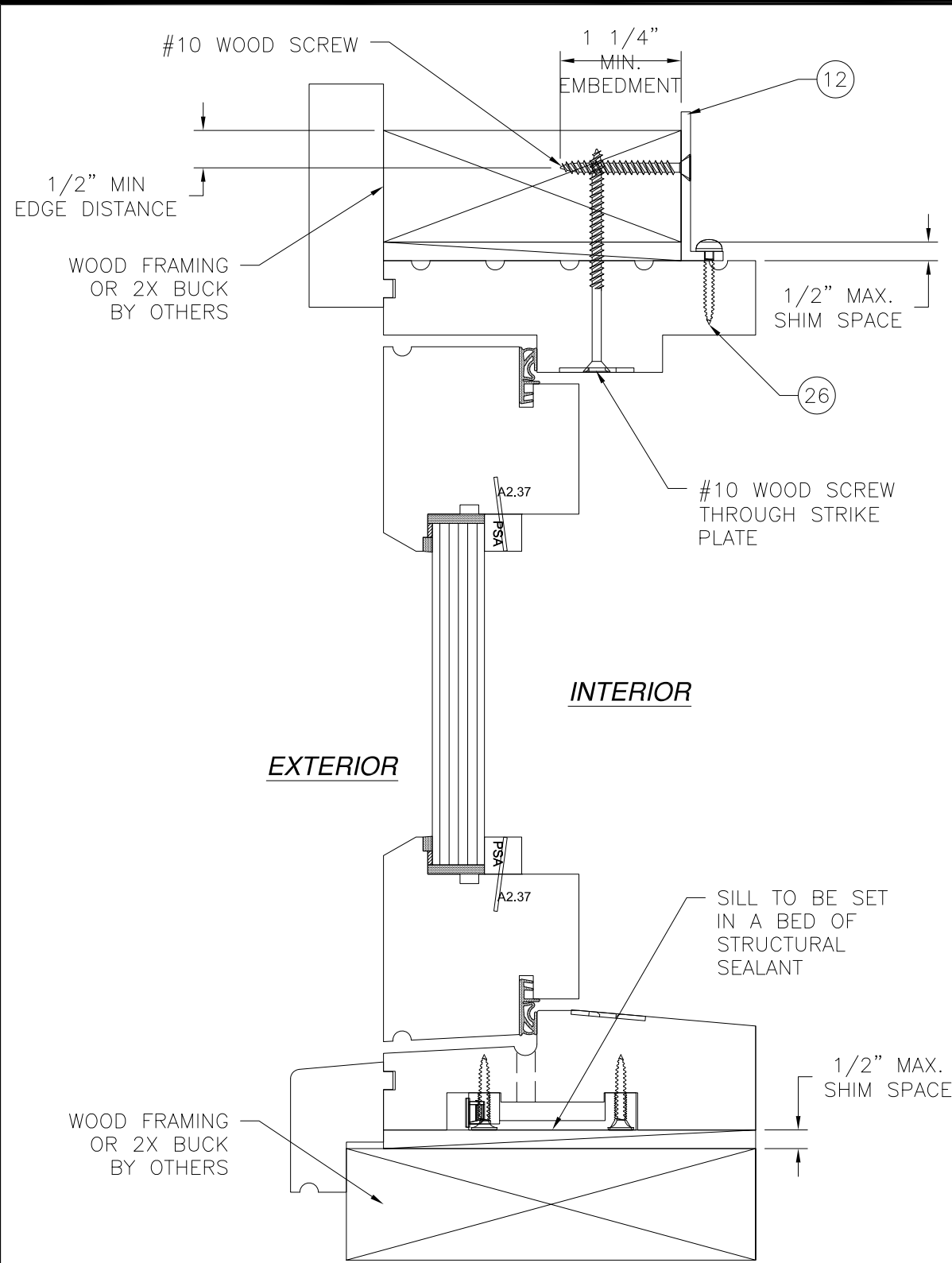
VERTICAL CROSS SECTION WOOD FRAMING OR 2X BUCK INSTALLATION STANDARD SILL SHOWN, SEE SHEET 20 FOR BRONZE SILL INSTALLATION
