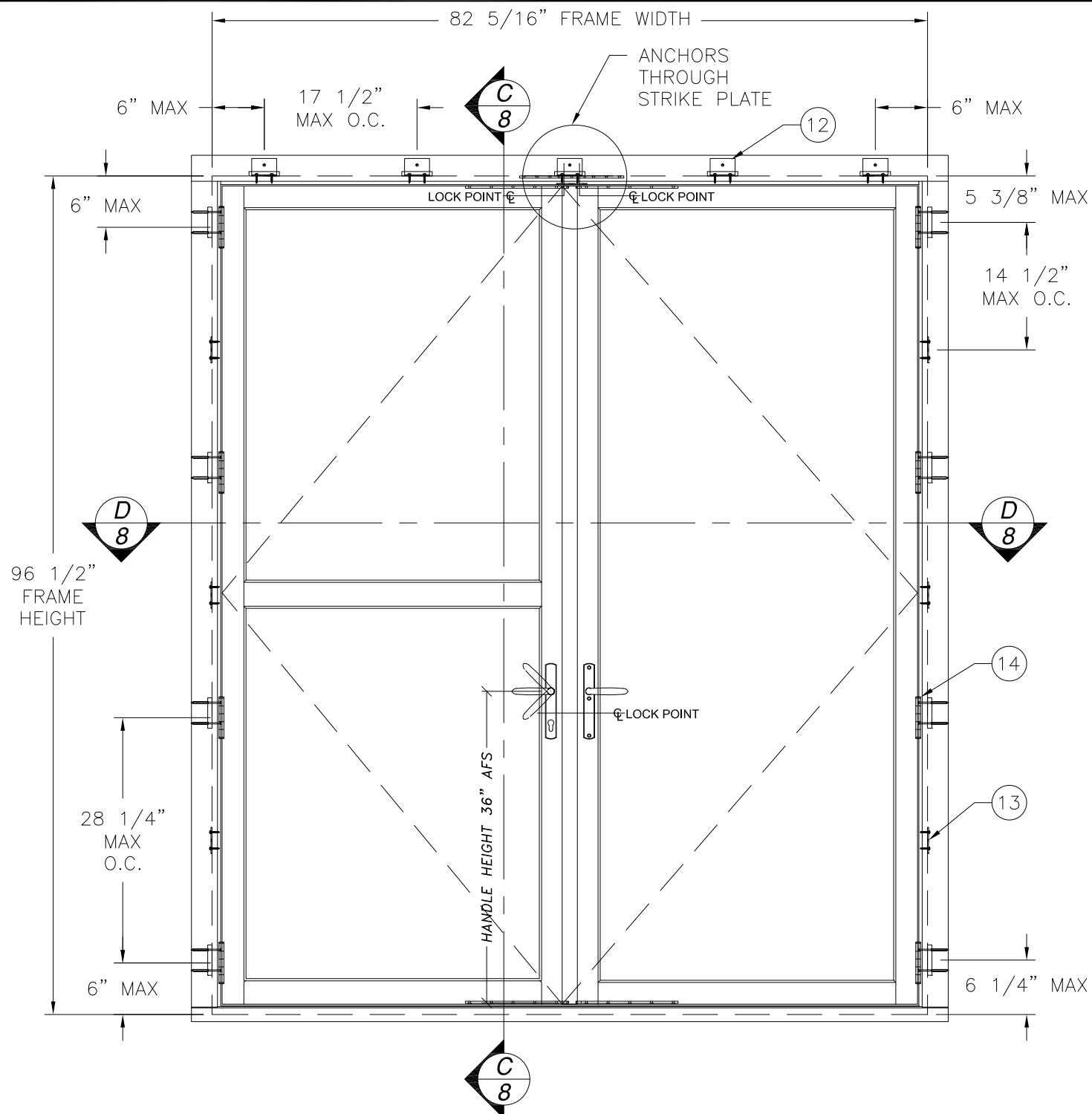
RWD WOOD FRENCH OUT-SWING DOUBLE DOOR EXTERIOR VIEW WITH MULTI POINT HOPPE LOCKING SYSTEM
