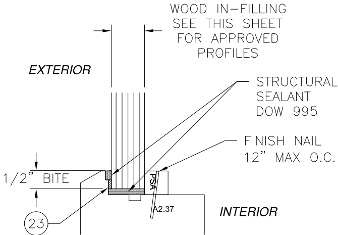
IN-FILLING DETAIL
