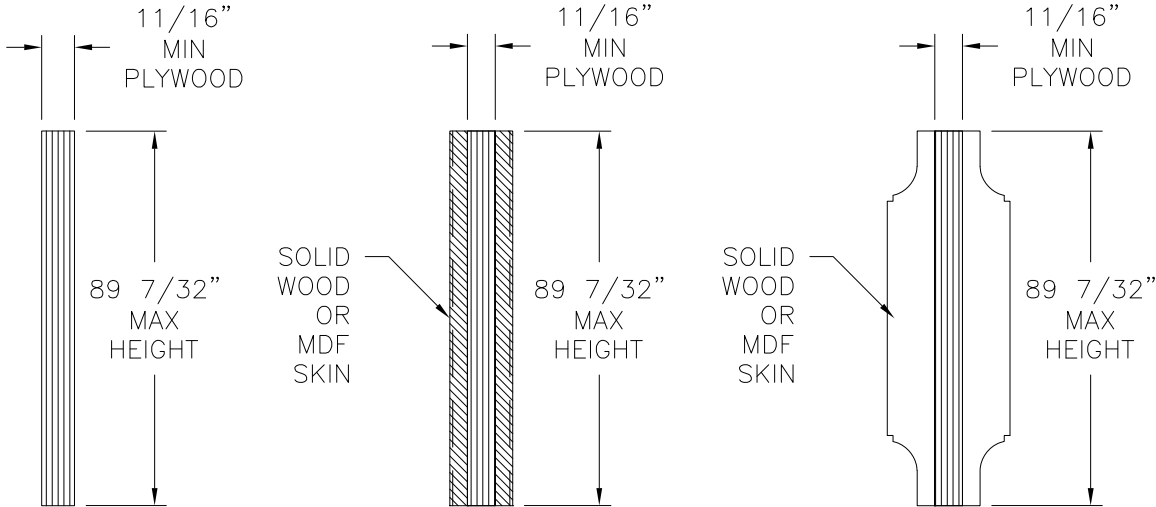
APPROVED IN-FILL PROFILES
