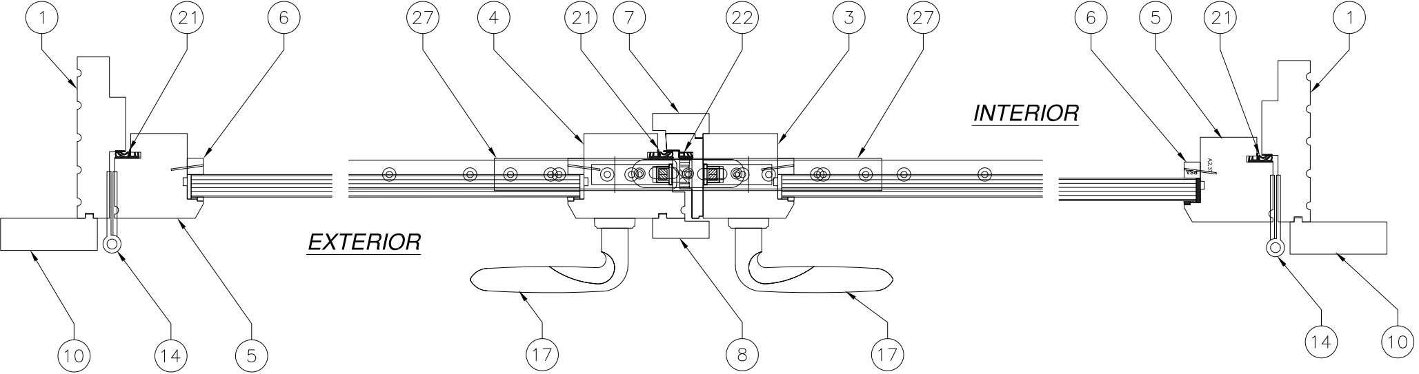
D 8 HORIZONTAL SECTION
