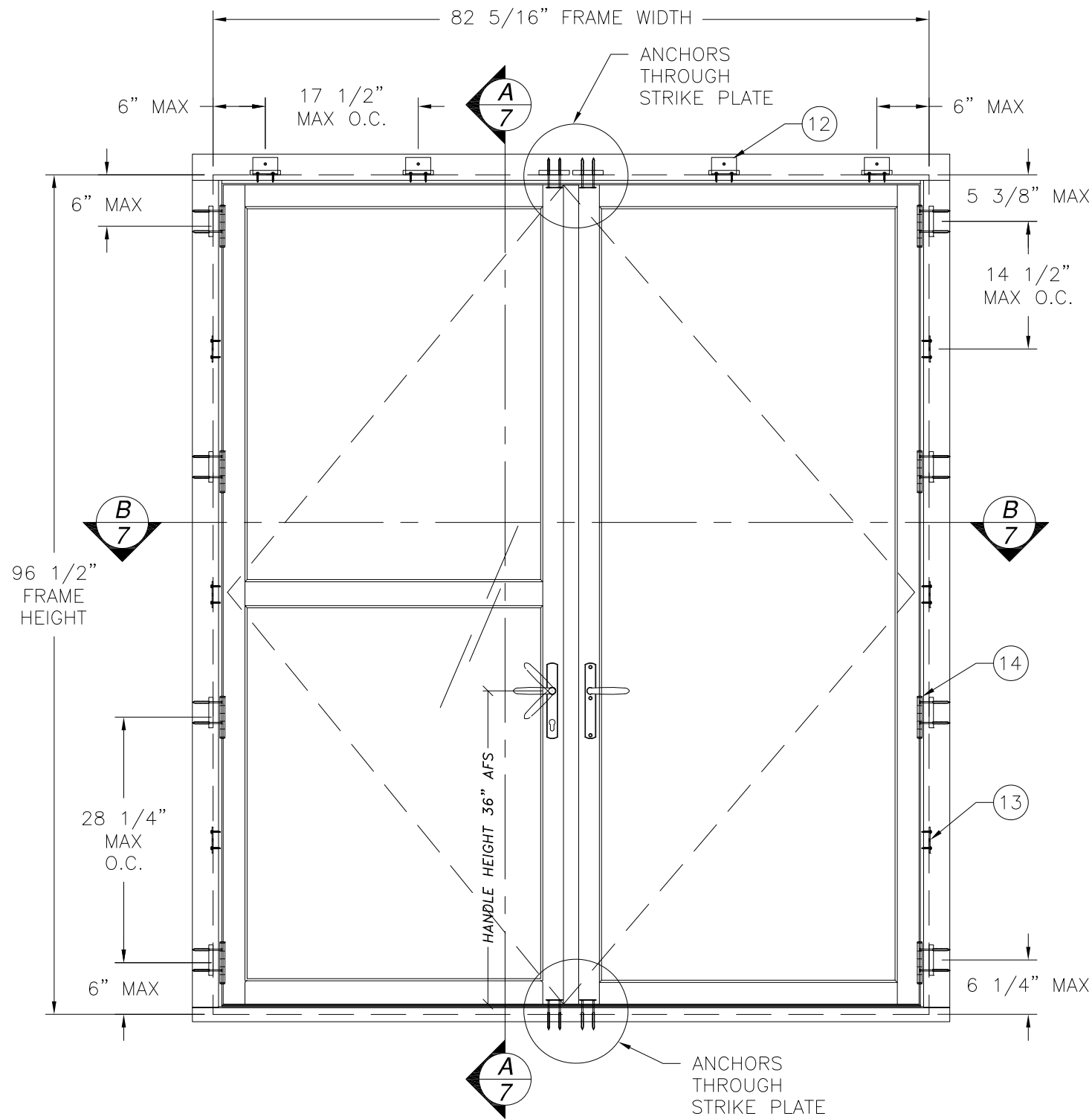
RWD WOOD FRENCH OUT-SWING DOUBLE DOOR EXTERIOR VIEW WITH SINGLE POINT ACCURATE LOCKING SYSTEM
