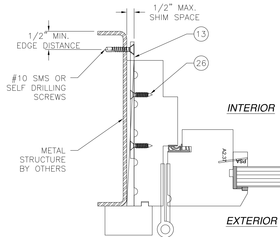
HORIZONTAL CROSS SECTION METAL STRUCTURE INSTALLATION
