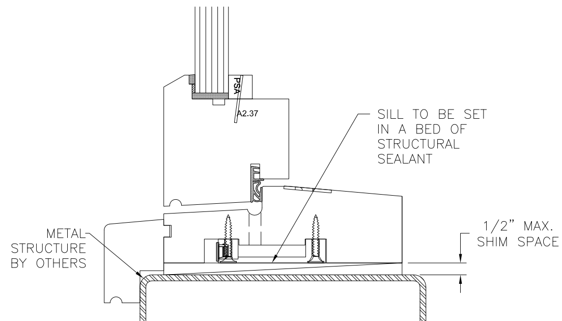
VERTICAL CROSS SECTION METAL STRUCTURE INSTALLATION STANDARD SILL SHOWN, SEE SHEET 20 FOR BRONZE SILL INSTALLATION
