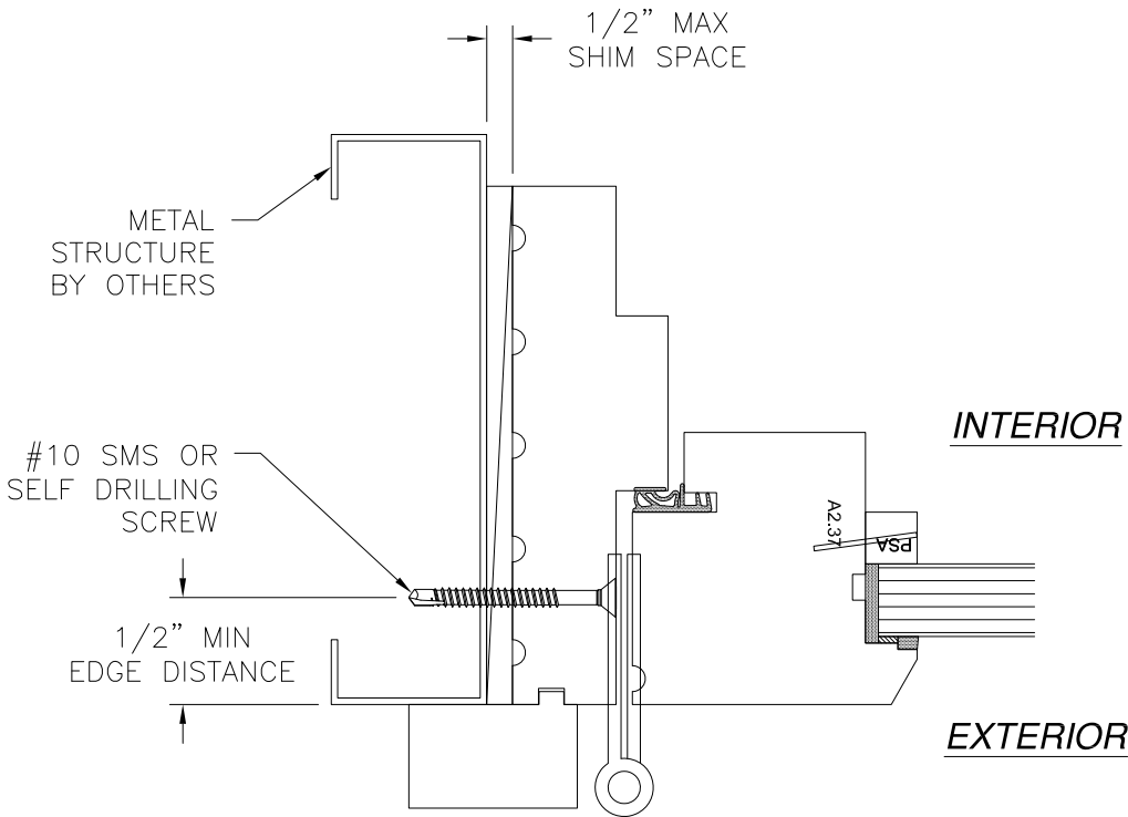
HORIZONTAL CROSS SECTION METAL STRUCTURE INSTALLATION
