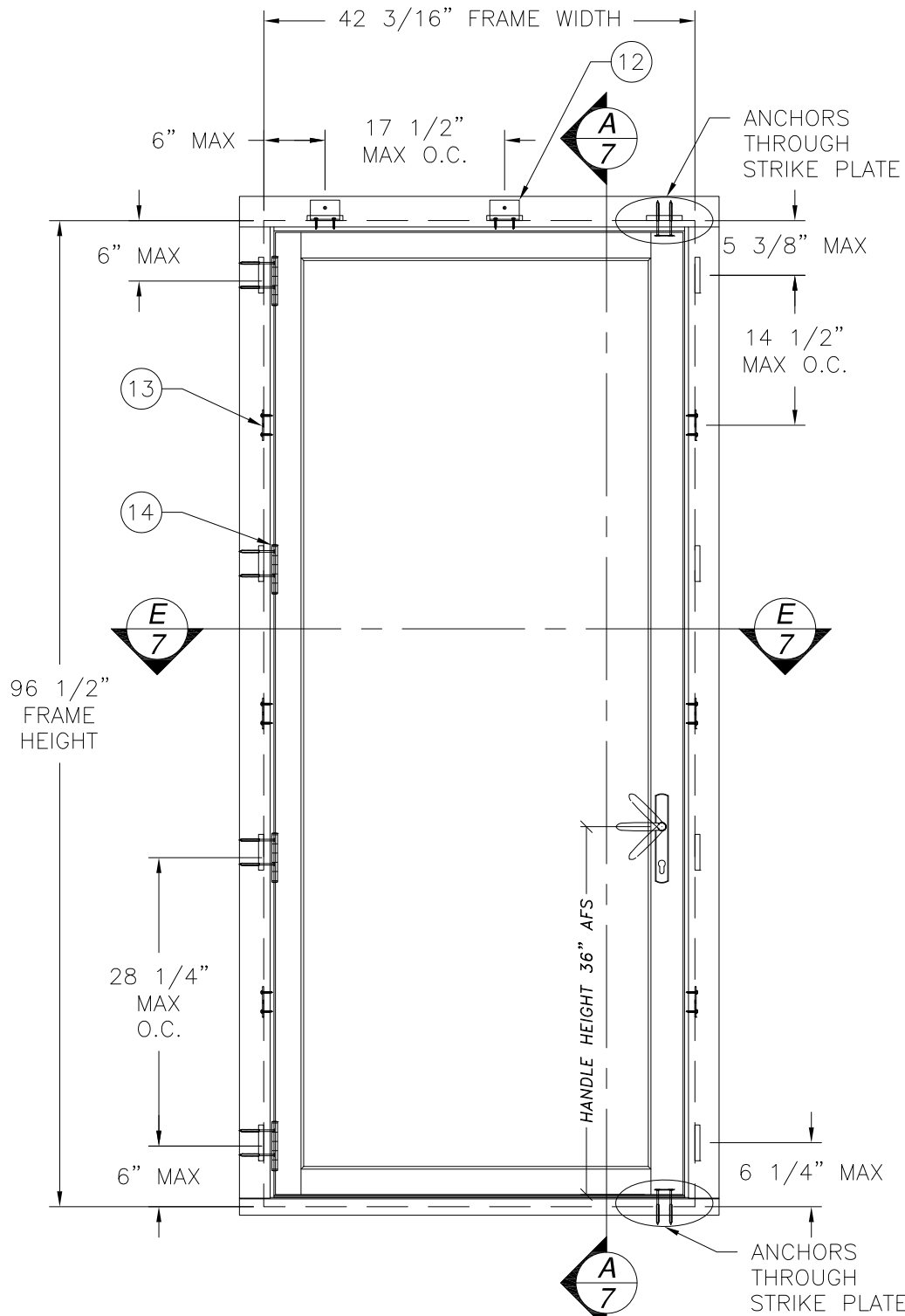
RWD WOOD FRENCH OUT-SWING SINGLE DOOR EXTERIOR VIEW WITH SINGLE POINT ACCURATE LOCKING SYSTEM
