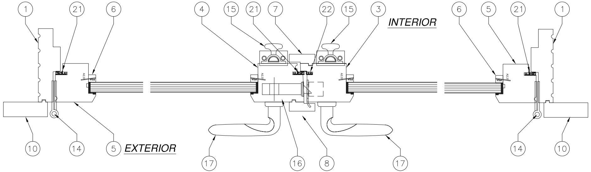
B 7 HORIZONTAL SECTION
