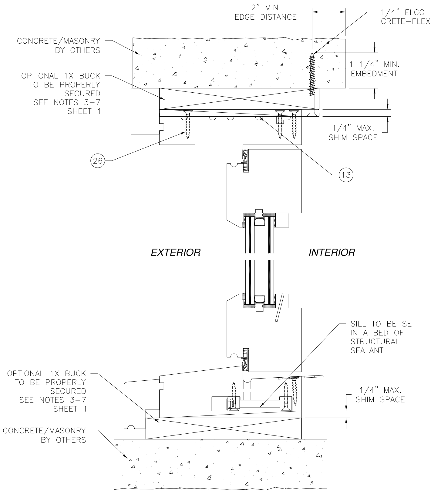
VERTICAL CROSS SECTION CONCRETE/MASONRY INSTALLATION WOOD SILL SHOWN, FOR BRONZE SILL INSTALLATION SEE SHEETS 20 AND 21
