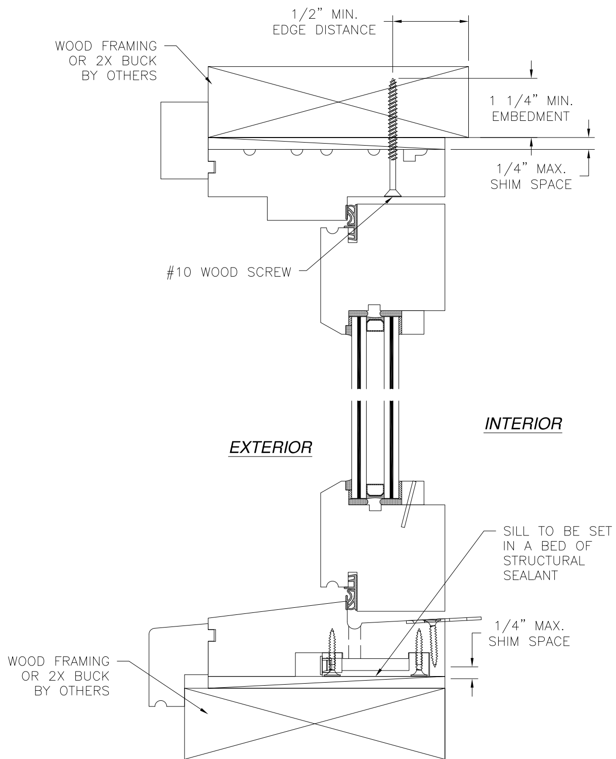
VERTICAL CROSS SECTION WOOD FRAMING OR 2X BUCK INSTALLATION WOOD SILL SHOWN, FOR BRONZE SILL INSTALLATION SEE SHEETS 20 AND 21
