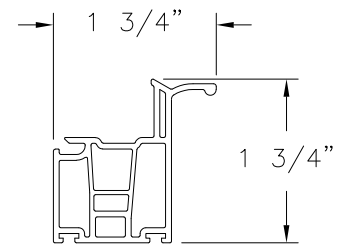
BOTTOM SASH BOTTOM RAIL RIGID PVC (V-1005)
