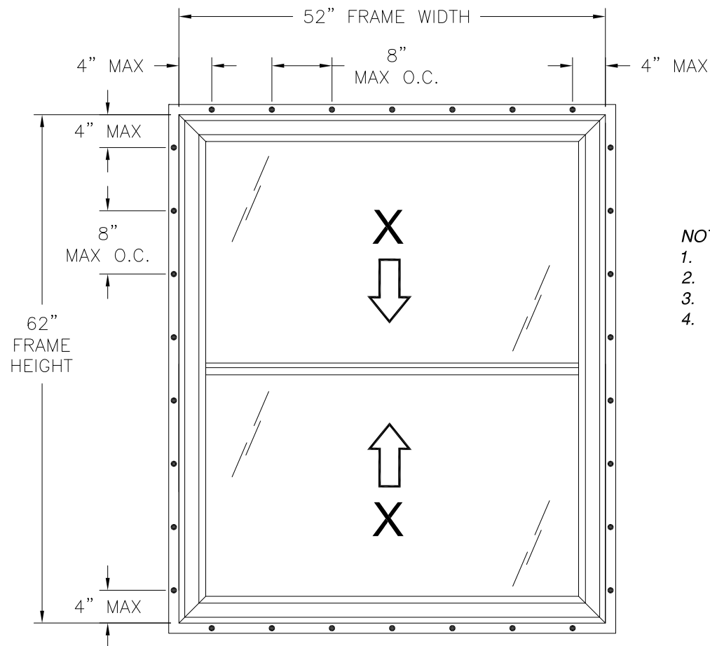
SERIES 1650 DOUBLE HUNG WINDOW FIN INSTALLATION
