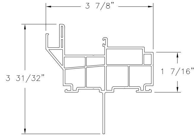
HEAD FRAME FIN INSTALLATION RIGID PVC (V-1028)
