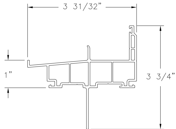
SILL FRAME FIN INSTALLATION RIGID PVC (V-1038)
