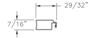
MEETING RAIL LINER STEEL, THICKNESS .019" (RF-104S-020)
