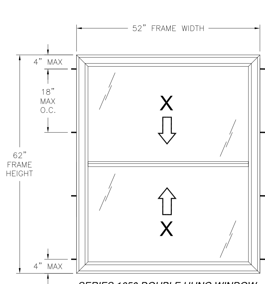
SERIES 1650 DOUBLE HUNG WINDOW FRAME INSTALLATION
