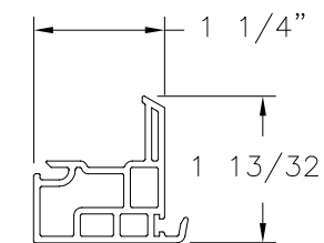
TOP SASH BOTTOM RAIL RIGID PVC (V-674)
