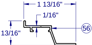
Screen, Interlock - 2097
