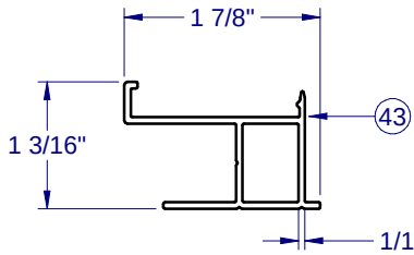
Screen, 1-Track Head/Jamb - 2135
