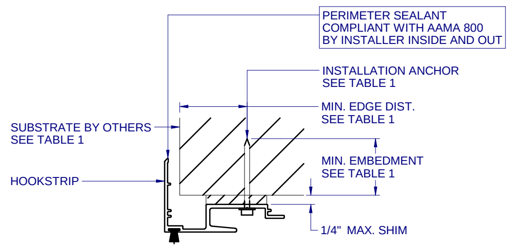
C 9 HORIZONTAL SECTION HOOK STRIP
