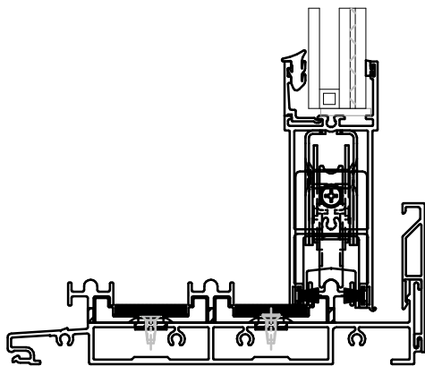
ALTERNATE SILL VIEW SILL RISER - 2094
