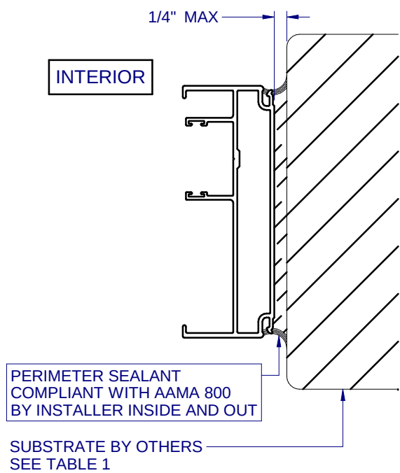
B 9 HORIZONTAL SECTION 2 TRACK JAMB ANCHORAGE
