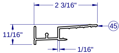
Screen, 1-Track Sill - 2134
