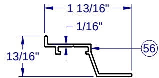
Screen, Interlock - 2097
