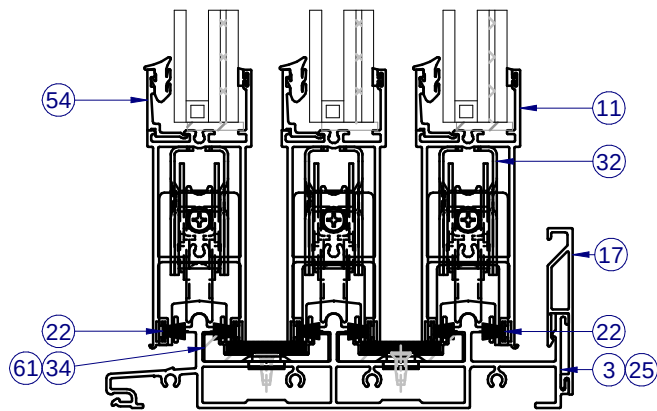
SECTION VIEW A-A DP +/- 65
