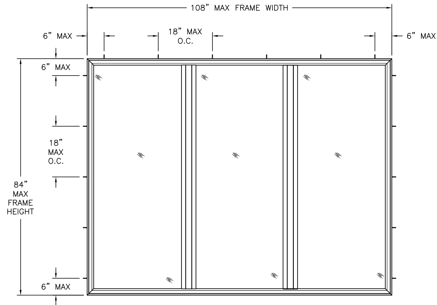
SERIES 4000 TRIPLE PICTURE WINDOW EXTERIOR VIEW FRAME INSTALLATION
