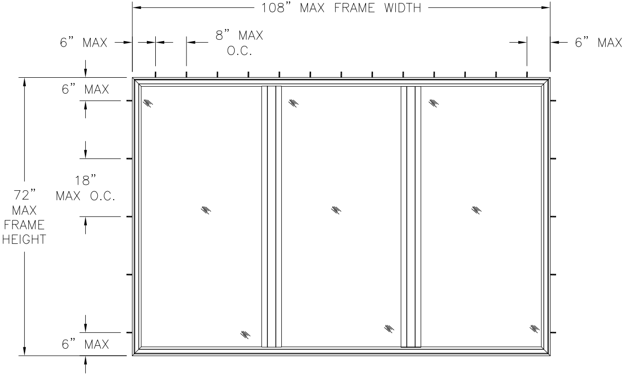
SERIES 400 TRIPLE PICTURE WINDOW EXTERIOR VIEW FRAME INSTALLATION
