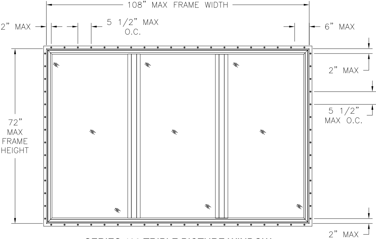
SERIES 400 TRIPLE PICTURE WINDOW EXTERIOR VIEW FIN INSTALLATION
