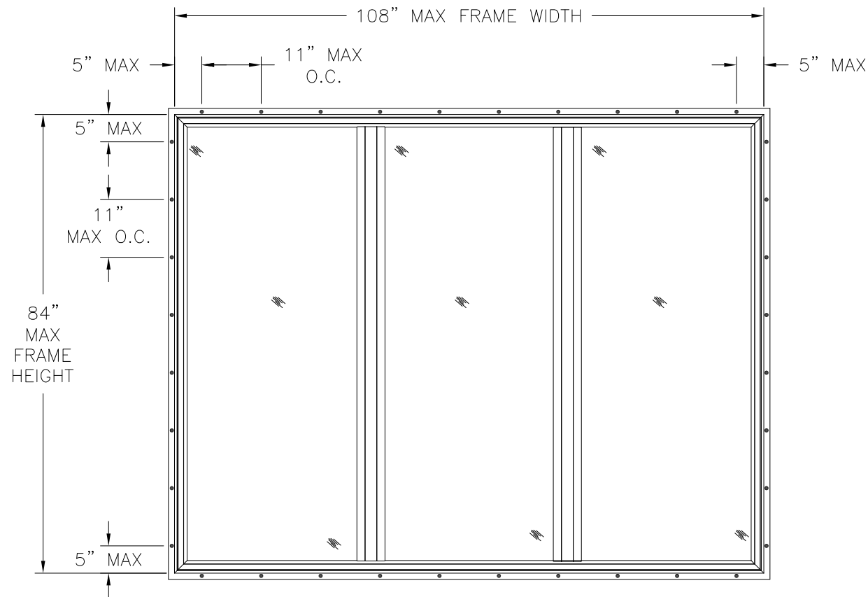
SERIES 400 TRIPLE PICTURE WINDOW EXTERIOR VIEW FIN INSTALLATION
