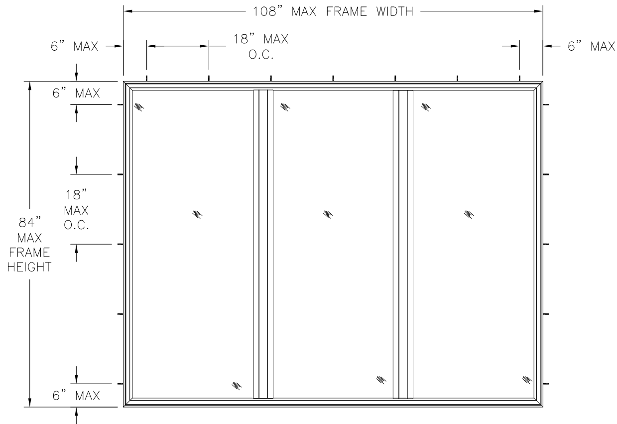
SERIES 400 TRIPLE PICTURE WINDOW EXTERIOR VIEW FRAME INSTALLATION
