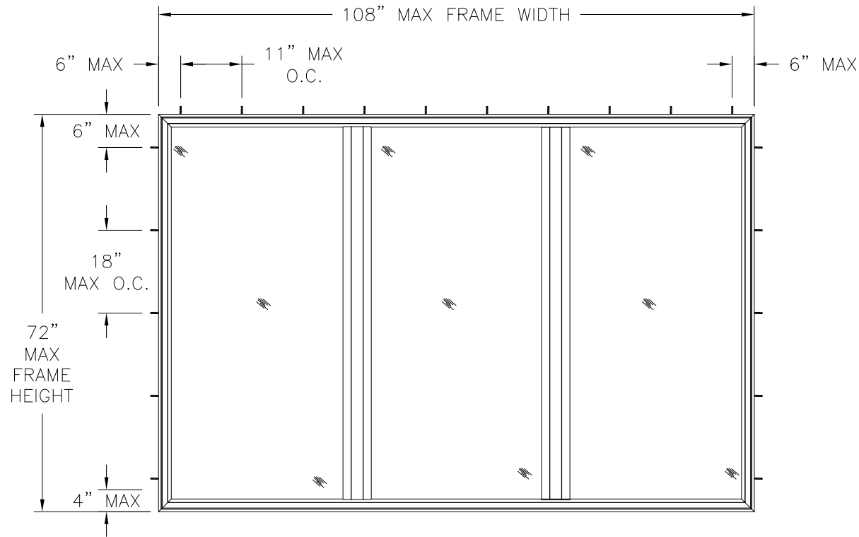
SERIES 400 TRIPLE PICTURE WINDOW EXTERIOR VIEW FRAME INSTALLATION
