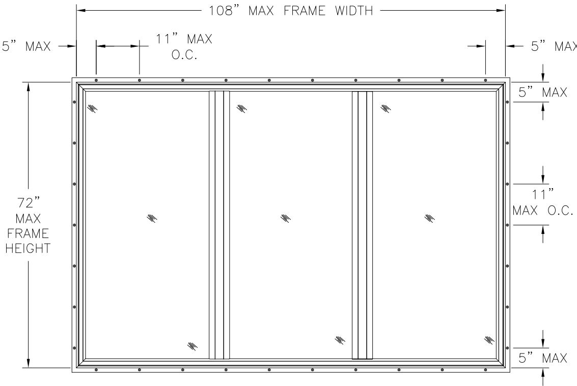
SERIES 400 TRIPLE PICTURE WINDOW EXTERIOR VIEW FIN INSTALLATION
