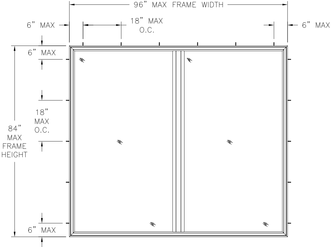
SERIES 400 TWIN PICTURE WINDOW EXTERIOR VIEW FRAME INSTALLATION
