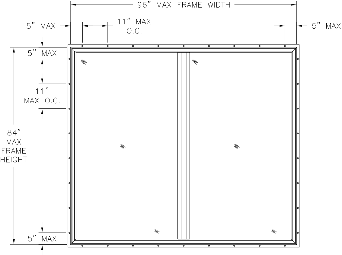
SERIES 400 TWIN PICTURE WINDOW EXTERIOR VIEW FIN INSTALLATION
