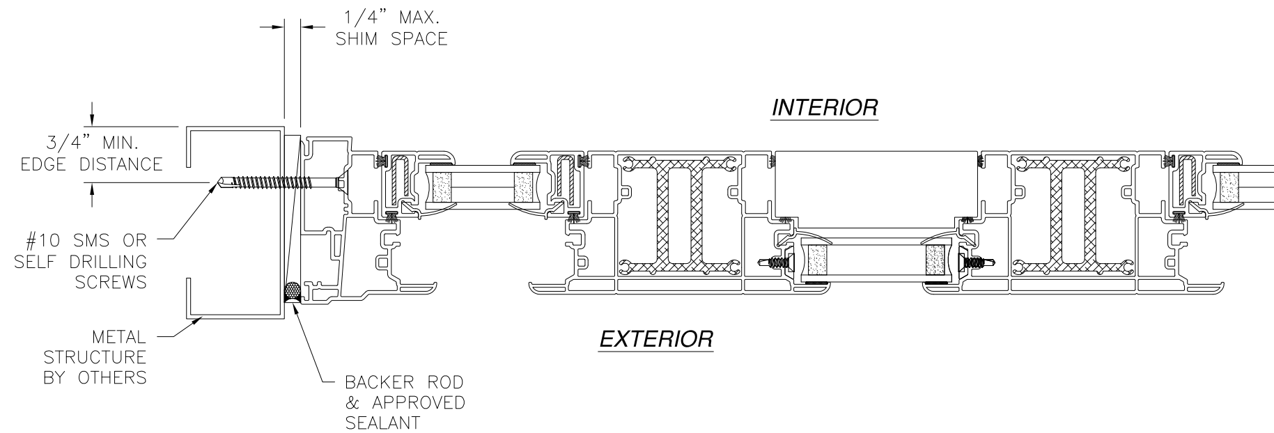
JAMB INSTALLATION DETAIL METAL STRUCTURE INSTALLATION
