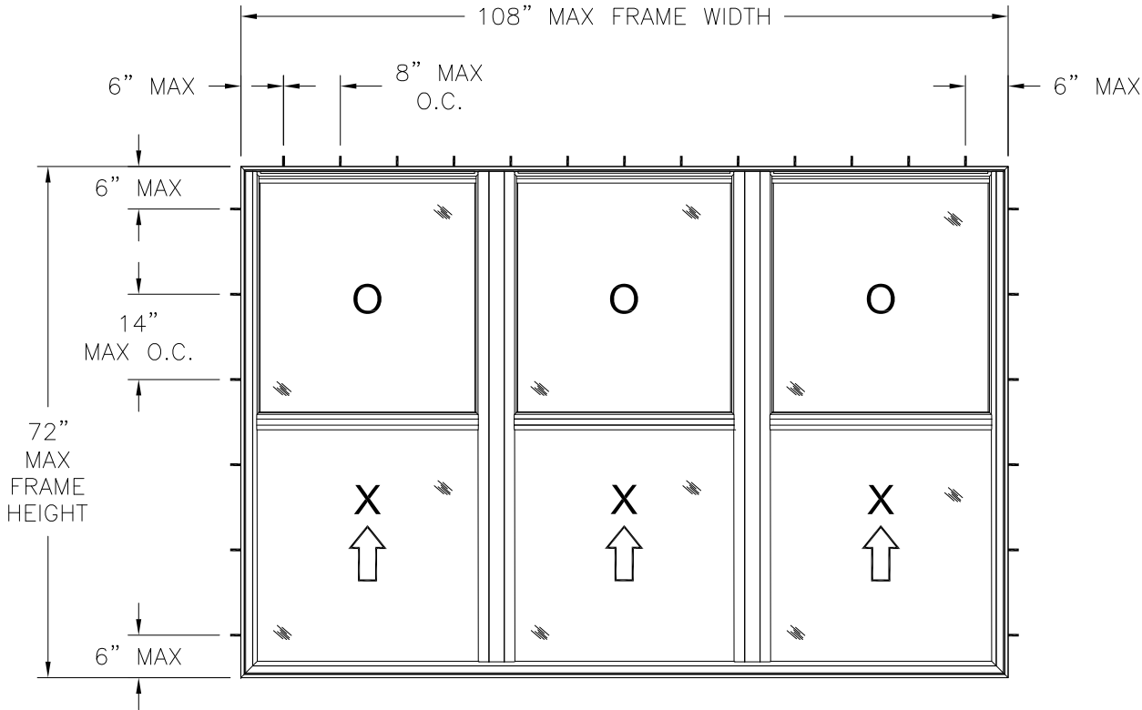
SERIES 400 TRIPLE SINGLE HUNG WINDOW EXTERIOR VIEW FRAME INSTALLATION
