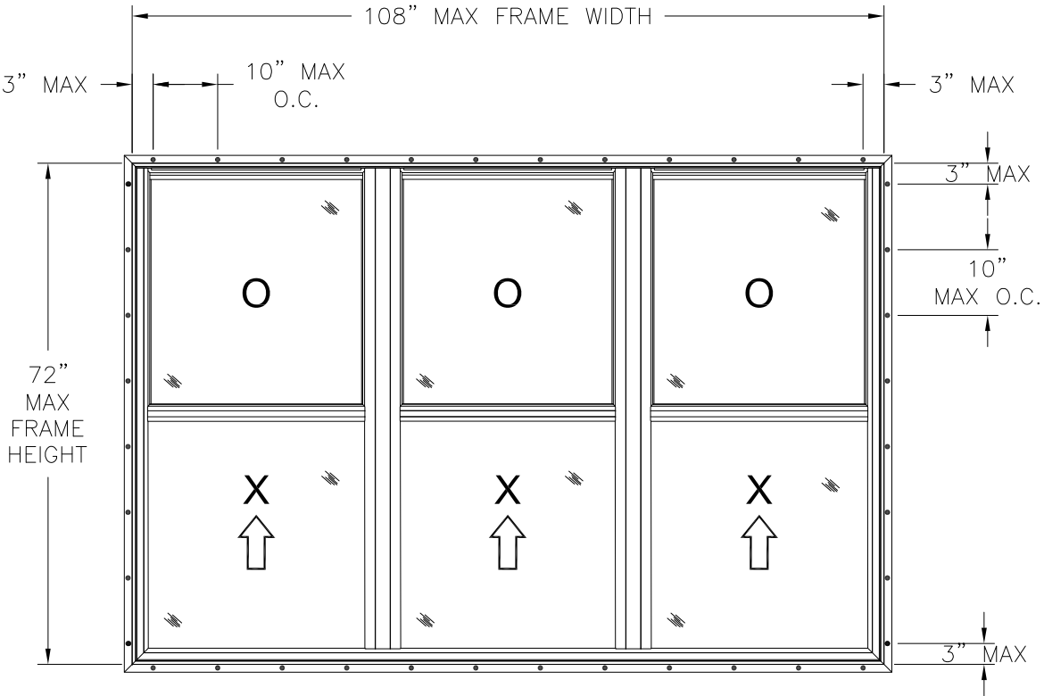
SERIES 400 TRIPLE SINGLE HUNG WINDOW EXTERIOR VIEW FIN INSTALLATION
