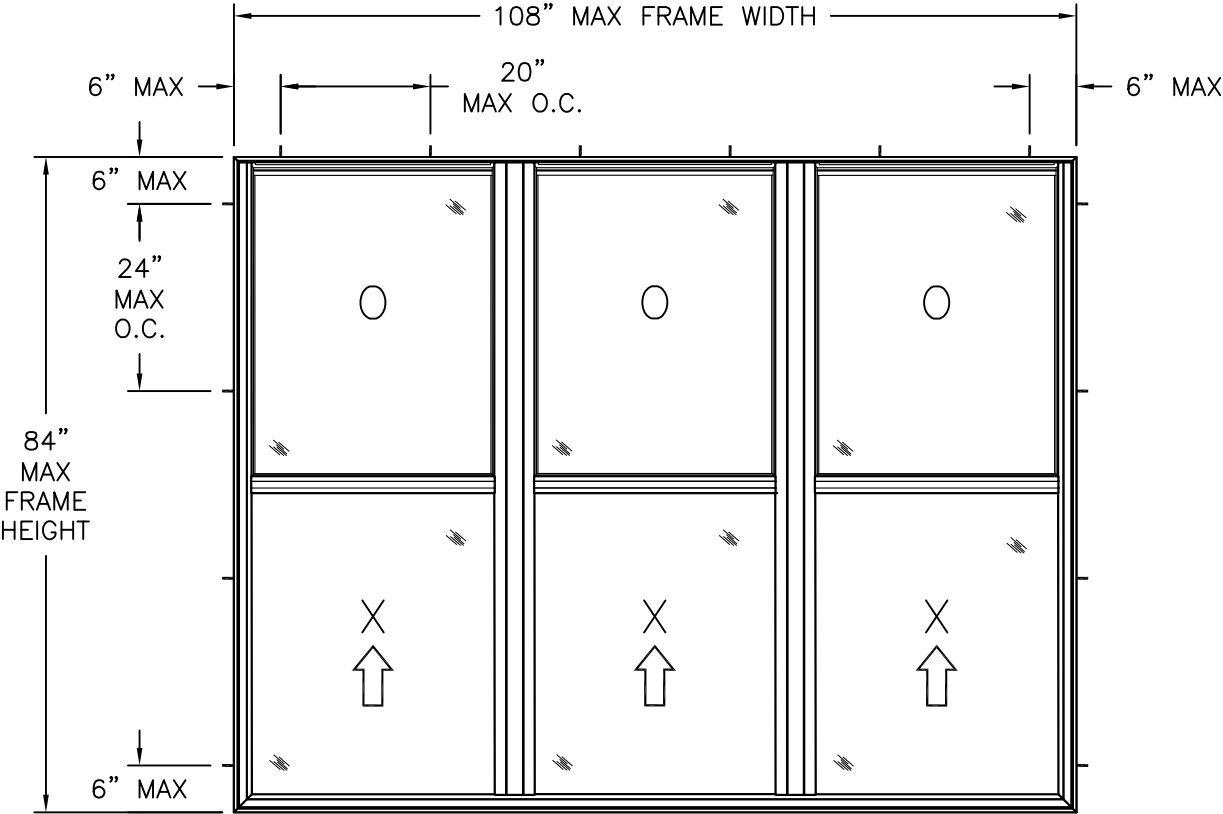
SERIES 4000 TRIPLE SINGLE HUNG WINDOW EXTERIOR VIEW FRAME INSTALLATION
