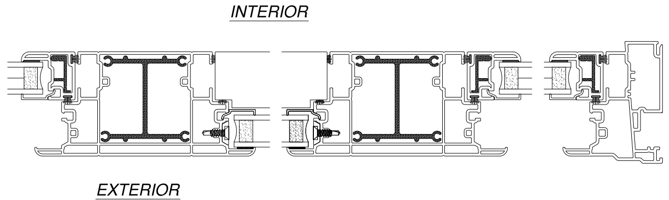
JAMB INSTALLATION DETAIL WOOD FRAMING OR 2X BUCK INSTALLATION
