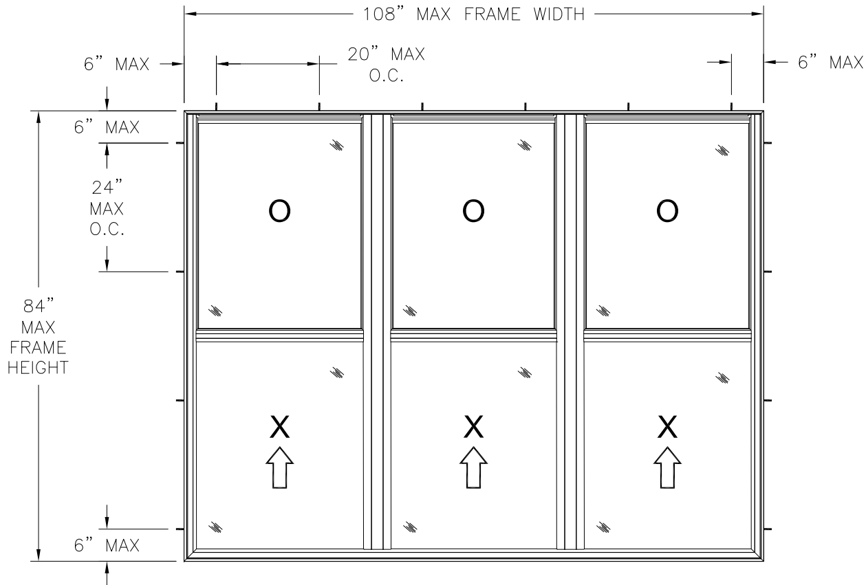
SERIES 400 TRIPLE SINGLE HUNG WINDOW EXTERIOR VIEW FRAME INSTALLATION
