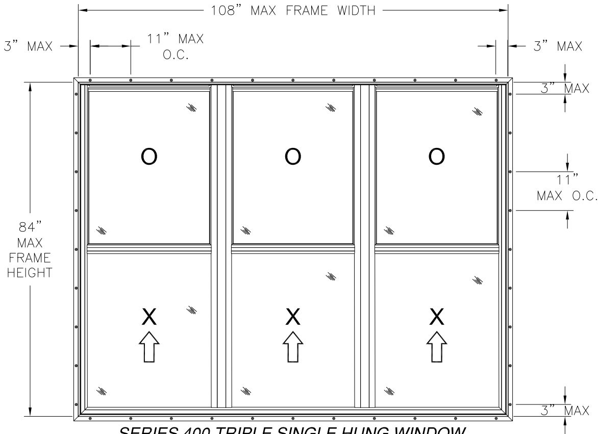
SERIES 400 TRIPLE SINGLE HUNG WINDOW EXTERIOR VIEW FIN INSTALLATION
