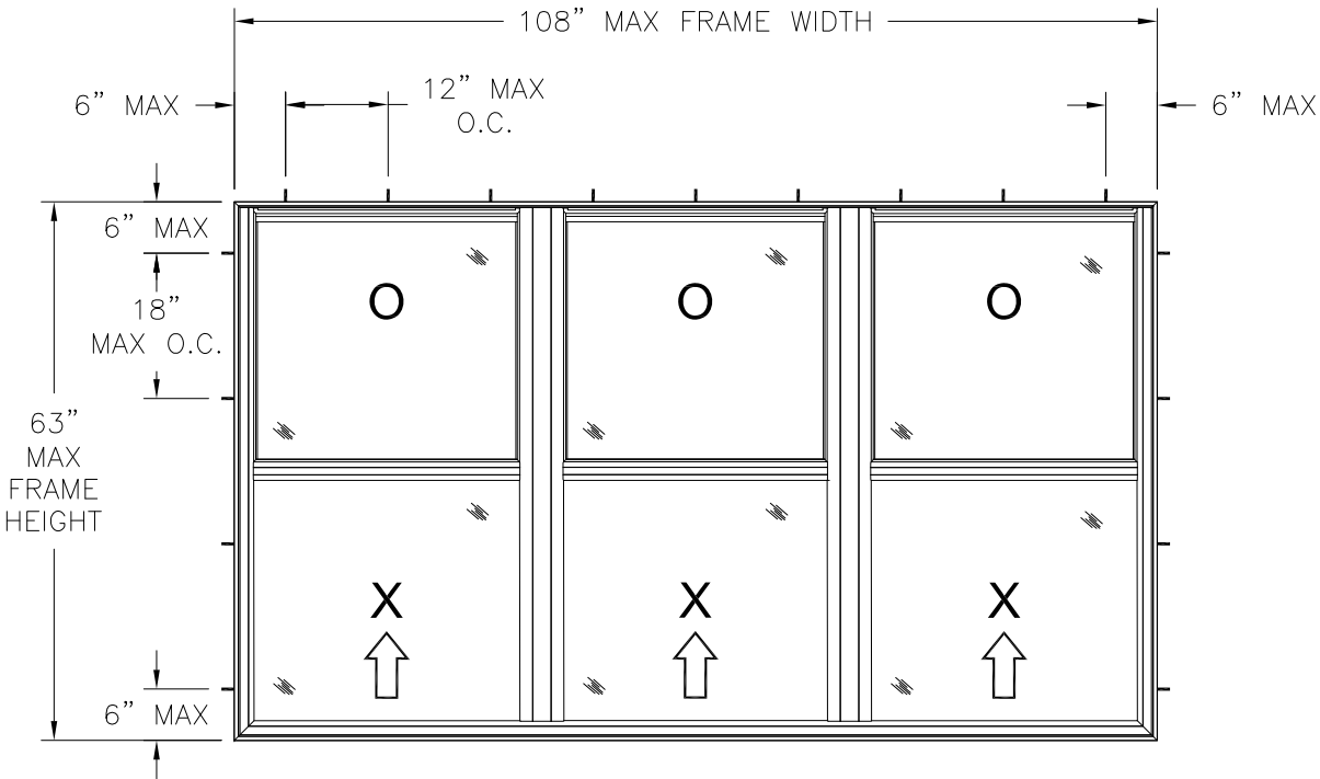
SERIES 400 TRIPLE SINGLE HUNG WINDOW EXTERIOR VIEW FRAME INSTALLATION
