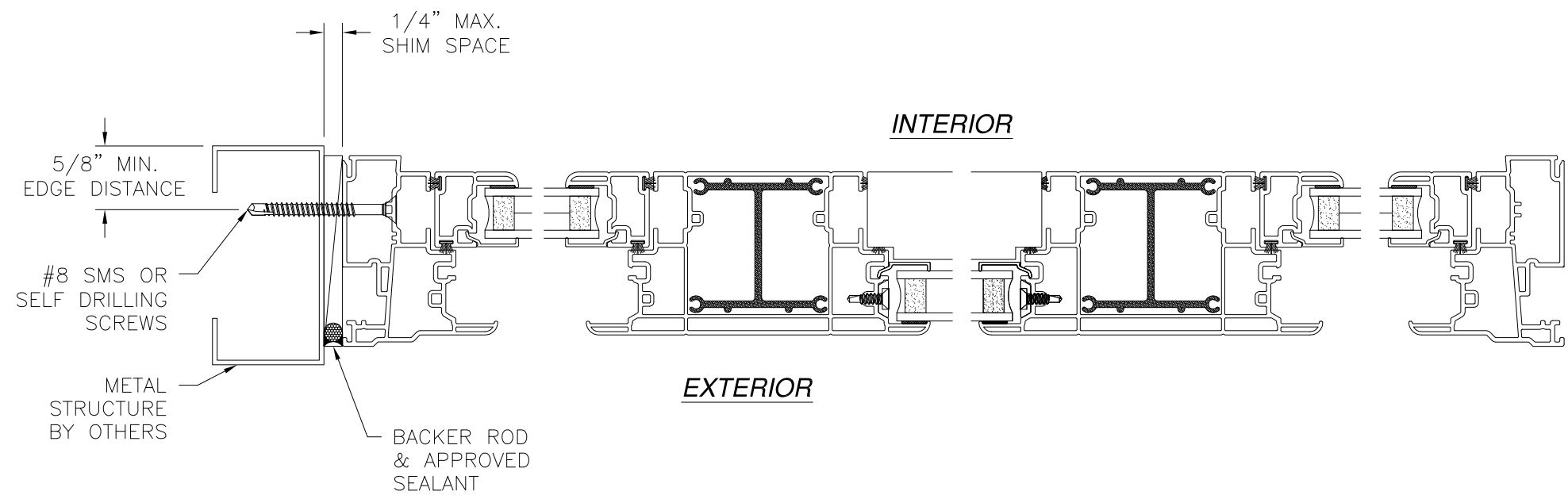
JAMB INSTALLATION DETAIL METAL STRUCTURE INSTALLATION
