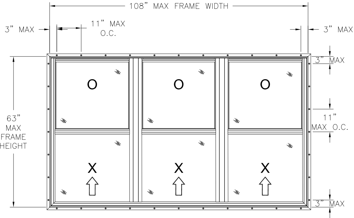
SERIES 400 TRIPLE SINGLE HUNG WINDOW EXTERIOR VIEW FIN INSTALLATION
