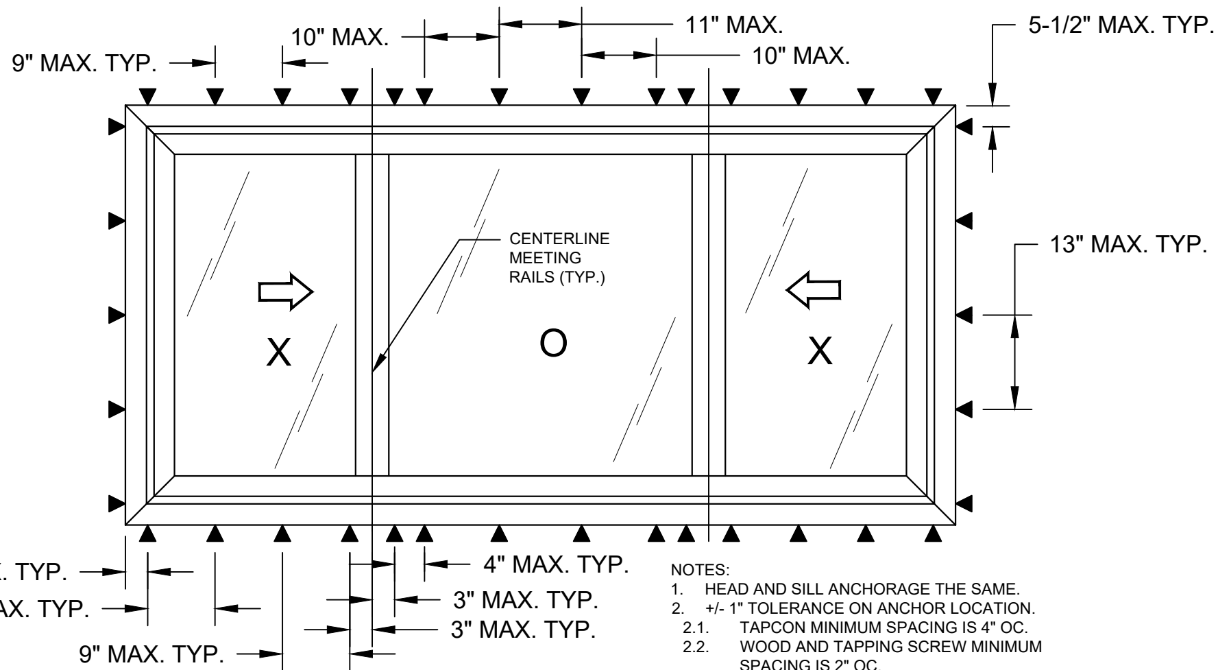
SERIES 5505 VINYL HORIZONTAL SLIDING XOX WINDOW EXTERIOR VIEW - ANCHORAGE
