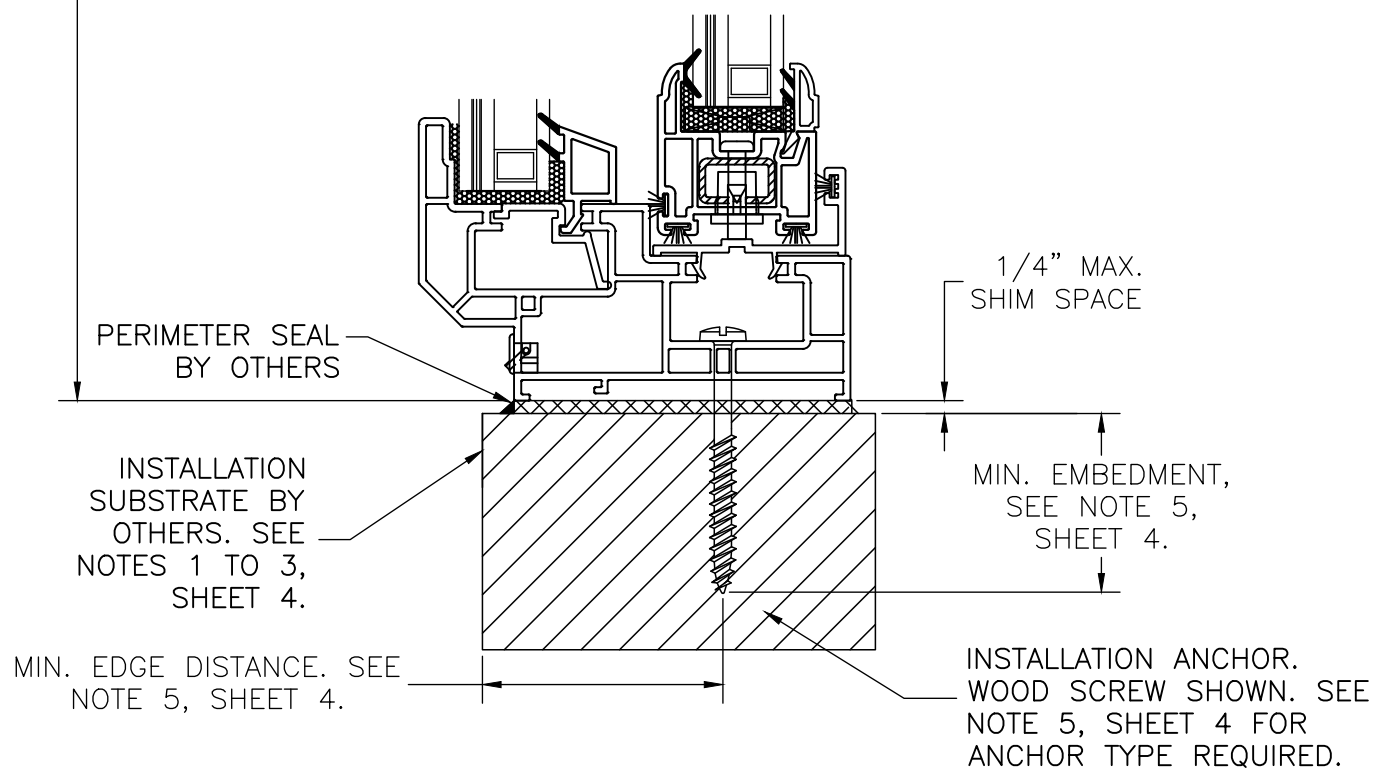
VERTICAL CROSS SECTION A-A WOOD FRAMING, 2X WOOD BUCK, CONCRETE/MASONRY OR METAL FRAME APPROVED
