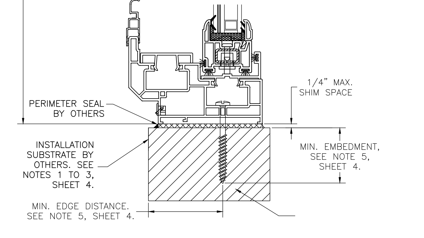
VERTICAL CROSS SECTION B-B WOOD FRAMING, 2X WOOD BUCK, CONCRETE/MASONRY OR METAL FRAME APPROVED
