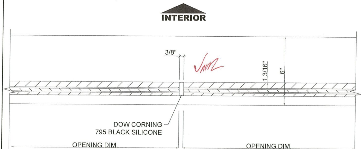
DETAIL A / IN-LINE MULTIPANEL SCALE: 3"=1'-0"
