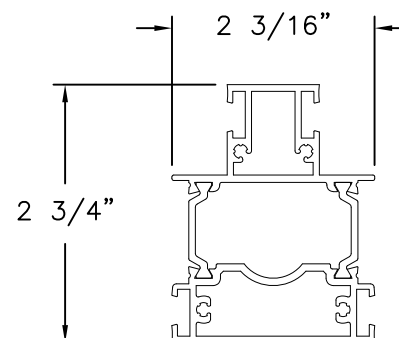
SLIDING POST ALUMINUM 6063-T5 .067" THICK
