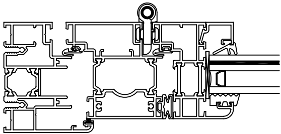
running carriage left side jamb
