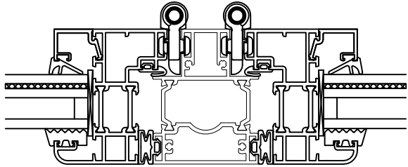
with running carriage set
