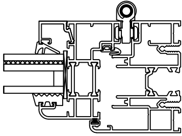
hinge at right side jamb
