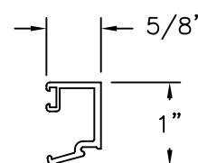
GLAZING BEAD ALUMINUM 6063-T5 .079" THICK
