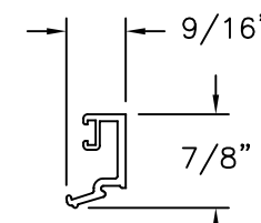
GLAZING BEAD ALUMINUM 6063-T5 .079" THICK
