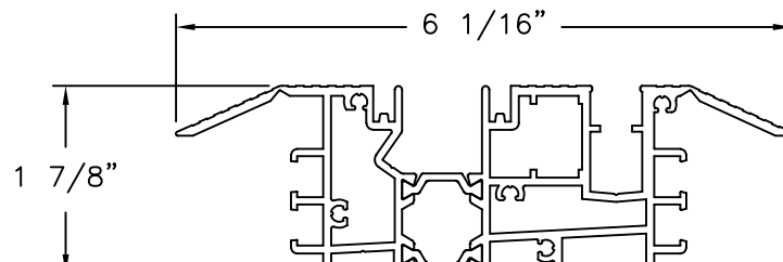
SADDLE SILL ALUMINUM 6063-T5 .077" THICK
