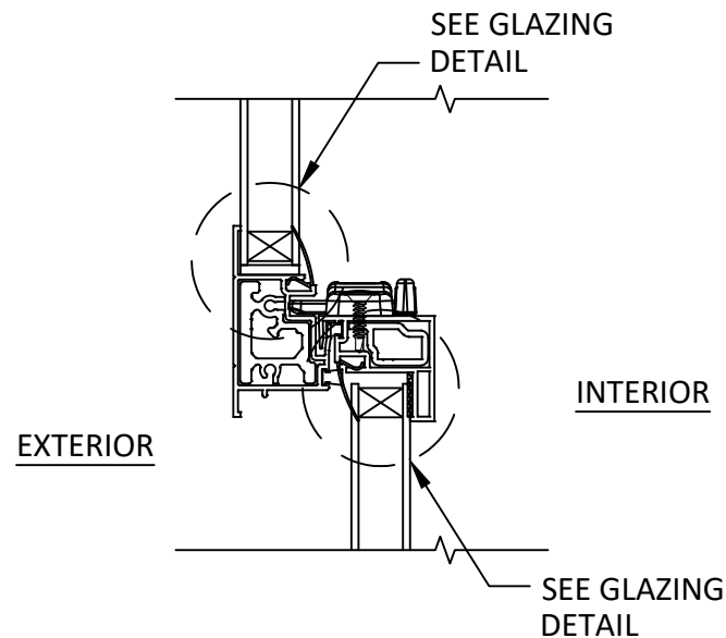
D 4 VERTICAL SECTION MEETING RAIL
