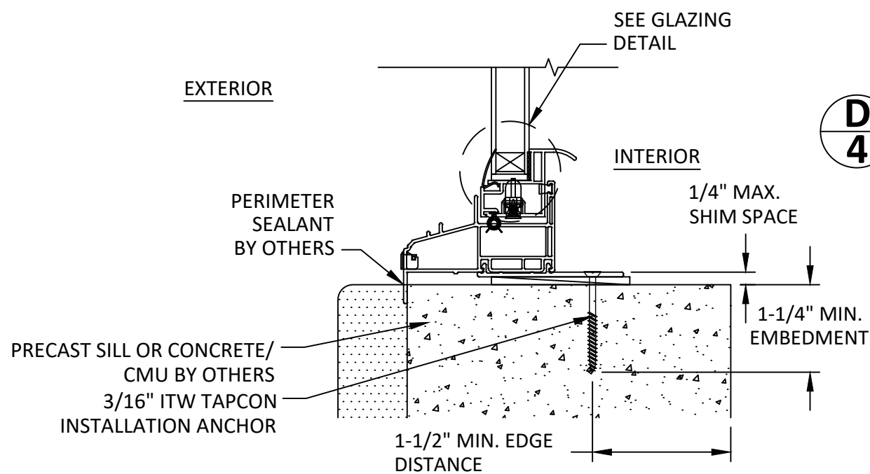
B 4 VERTICAL SECTION SILL WITH CLIP - CONCRETE/MASONRY
