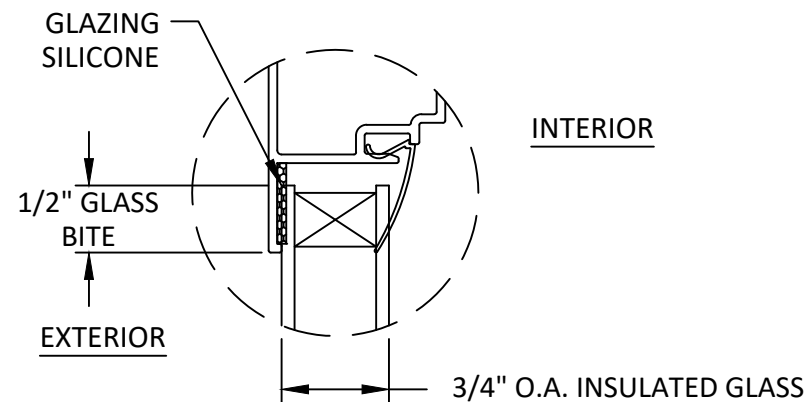
GLAZING DETAIL
