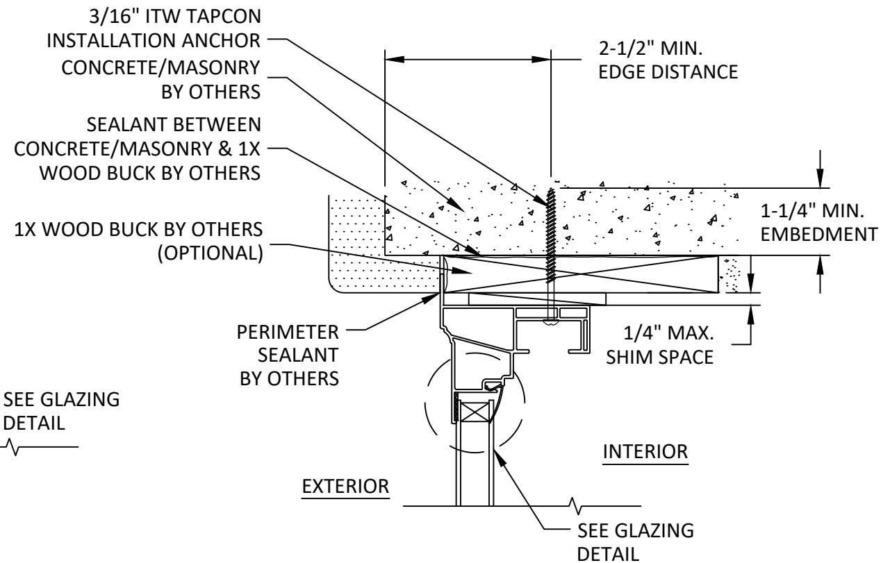
C 4 VERTICAL SECTION SINGLE HUNG HEAD - 1X/CONC./MASONRY
