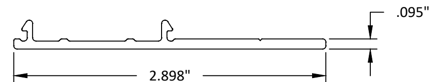
SILL CLIP
