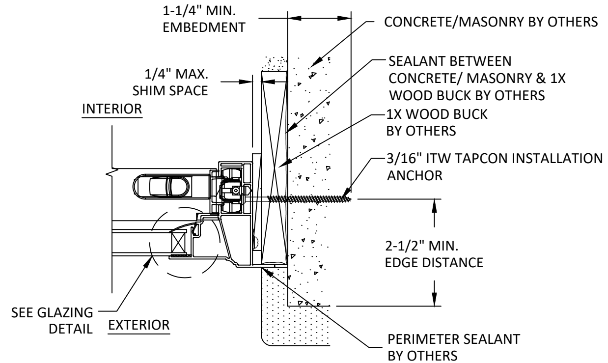
G5 HORIZONTAL SECTION SINGLE HUNG JAMB - 1X WOOD/CONC./MASONRY
