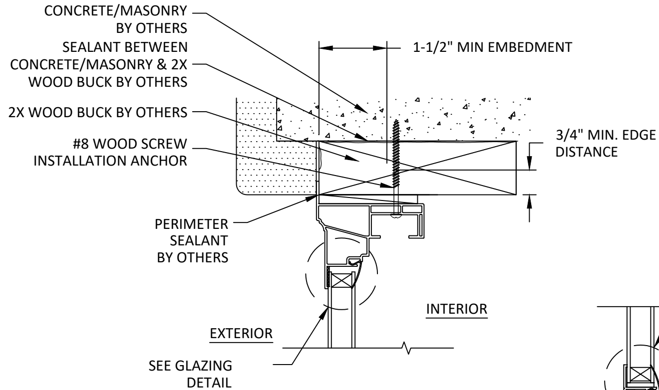
A 4 VERTICAL SECTION SINGLE HUNG HEAD - 2X WOOD BUCK
