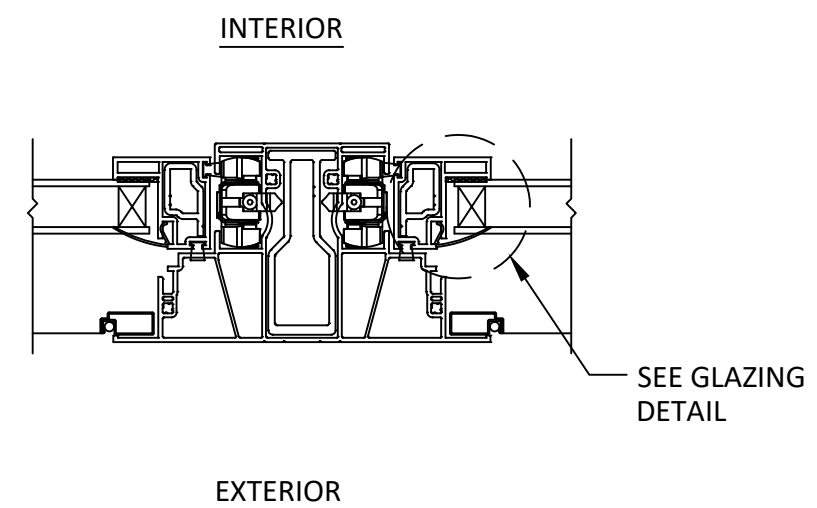
E 4 HORIZONTAL SECTION CONTINUOUS FRAME MULL BAR
