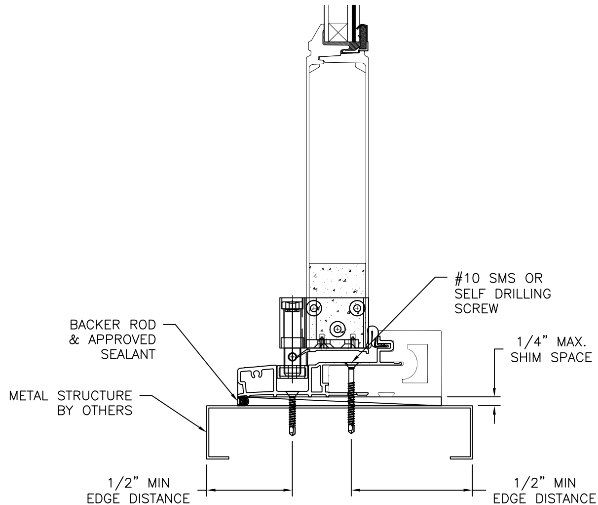
VERTICAL CROSS SECTION METAL STRUCTURE INSTALLATION
