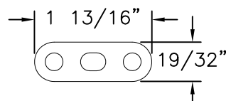
DRIVER BAR PLATE GASKET TPE SEE NOTE 6
