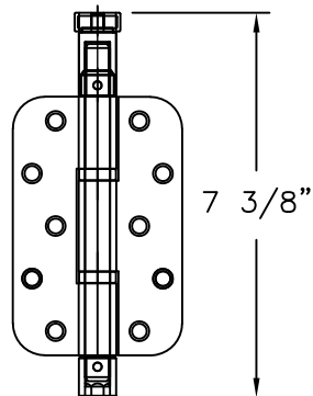
HINGE STEEL, POM SEE NOTE 2
