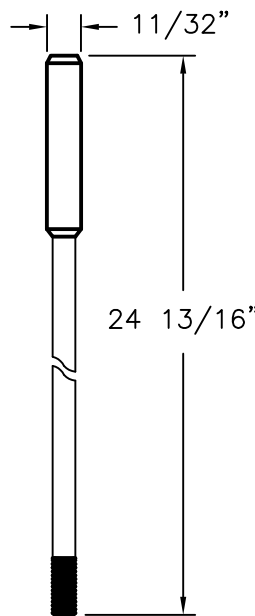
25" FLUSH BOLT BAR STAINLESS STEEL
