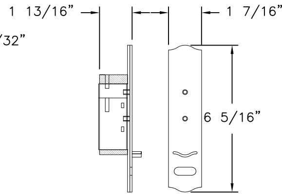
FLUSH BOLT MECHANISM DIE CAST STEEL ABS SEE NOTE 3
