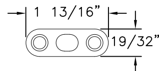
DRIVER BAR PLATE STAINLESS STEEL SEE NOTE 6
