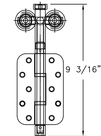
HINGE W/CARRIER STEEL, POM SEE NOTE 2
