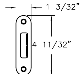
HOOK KEEPER STAINLESS STEEL SEE NOTE 4
