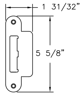
MULTI POINT LOCK KEEPER STAINLESS STEEL SEE NOTE 5
