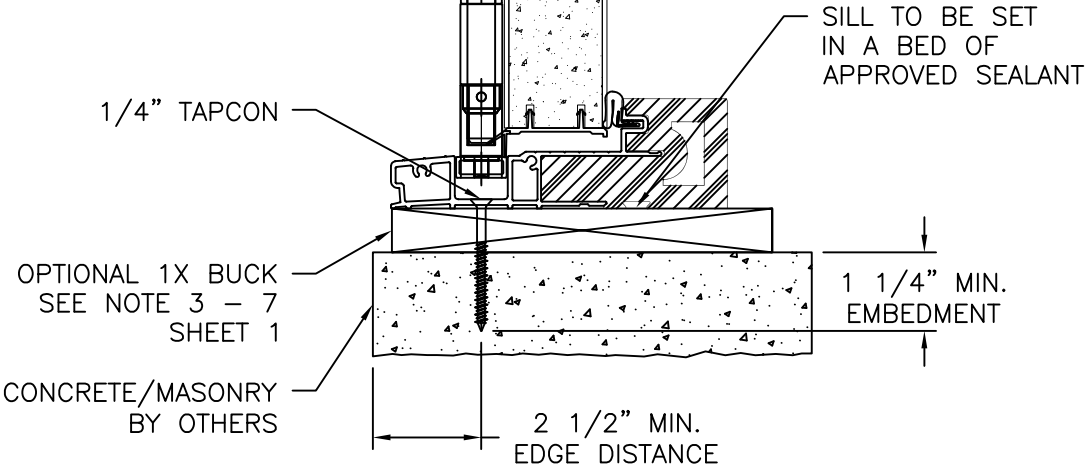
VERTICAL CROSS SECTION CONCRETE/MASONRY INSTALLATION
