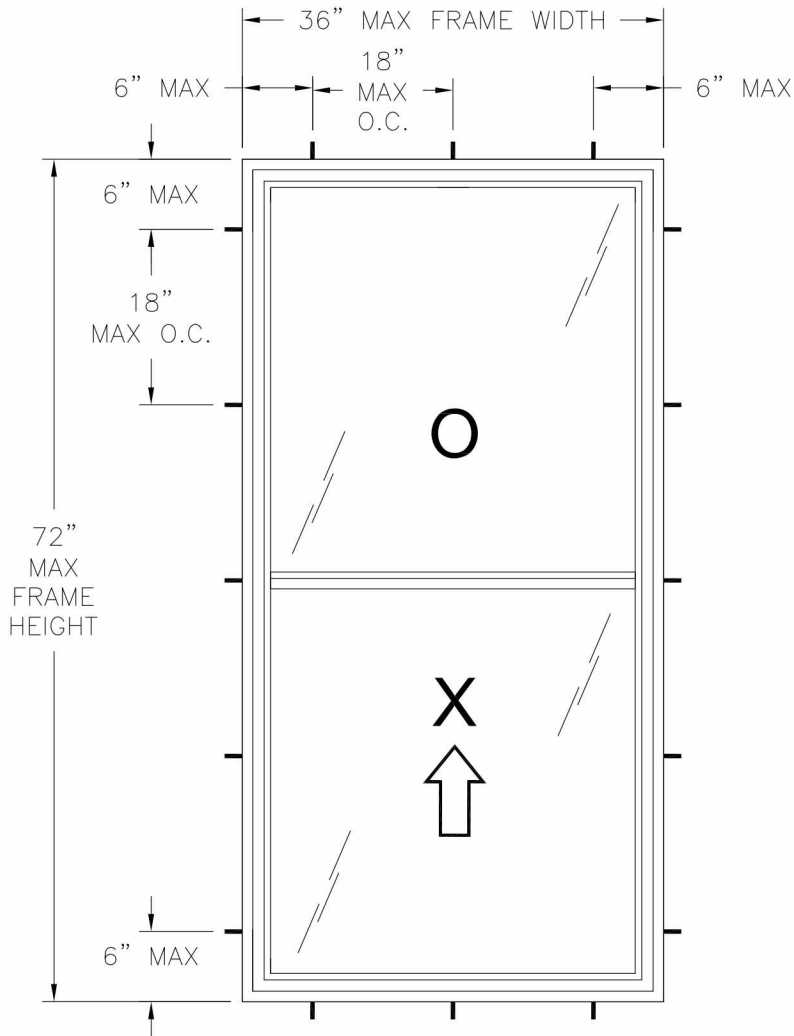
SERIES 900 VINYL SINGLE HUNG WINDOW EXTERIOR VIEW FRAME INSTALLATION
