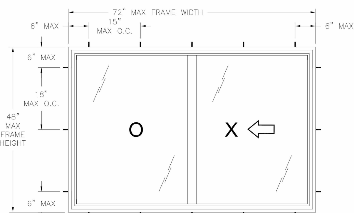
SERIES 920 VINYL HORIZONTAL SLIDING WINDOW EXTERIOR VIEW FRAME INSTALLATION
