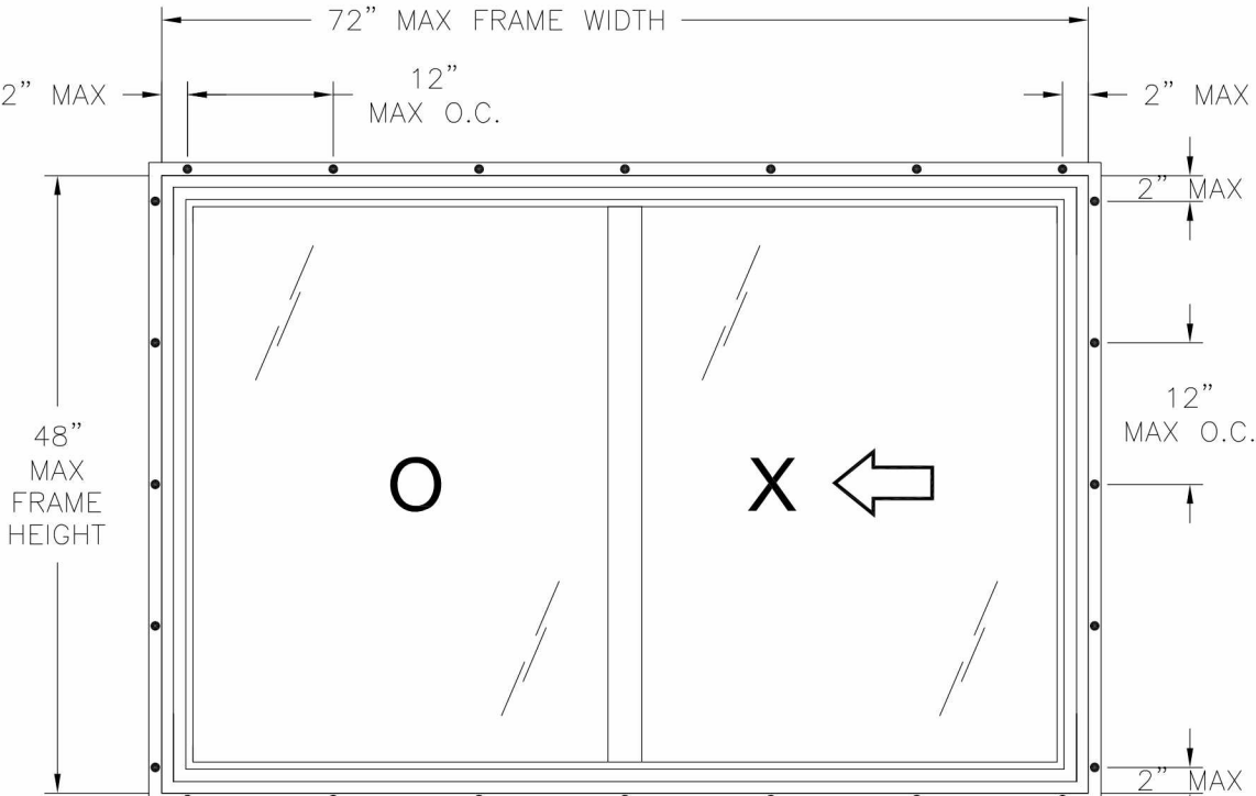
SERIES 920 VINYL HORIZONTAL SLIDING WINDOW EXTERIOR VIEW FIN INSTALLATION
