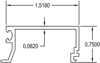
3 1" GLAZING BEAD SCALE 1:1
