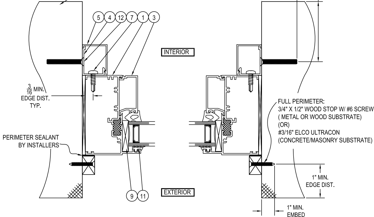
B HORIZONTAL SECTION SCALE 1:1
