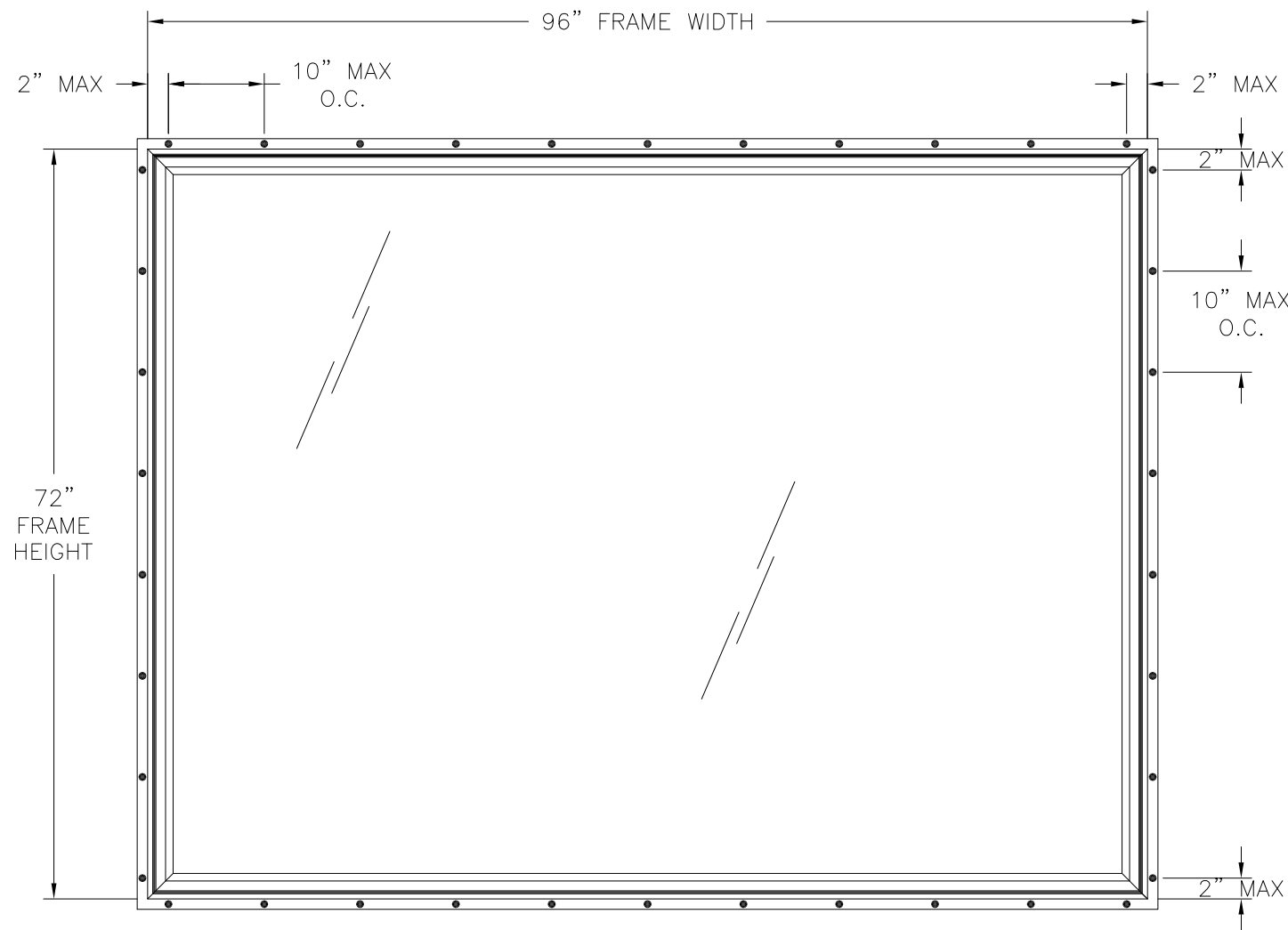
SERIES 3500 FIXED WINDOW EXTERIOR VIEW
