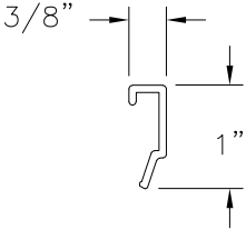
GLAZING BEAD PVC (V-819)
