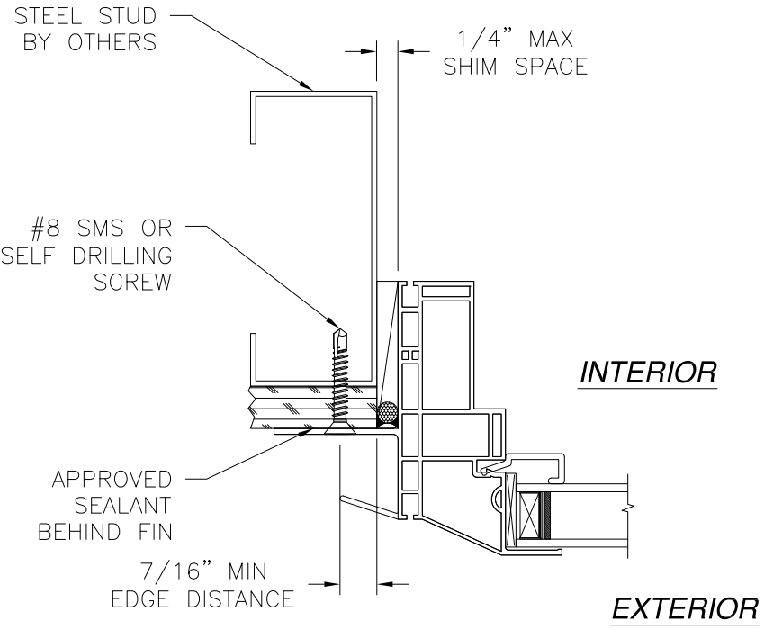
JAMB INSTALLATION DETAIL STEEL STUDS INSTALLATION
