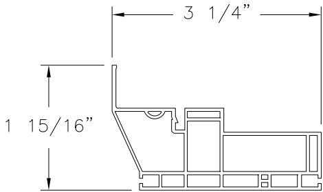
MAIN FRAME EXTRUDED RIGID PVC (V-915)
