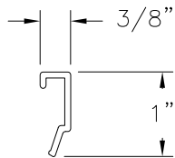
GLAZING BEAD EXTRUDED RIGID PVC (V-819)
