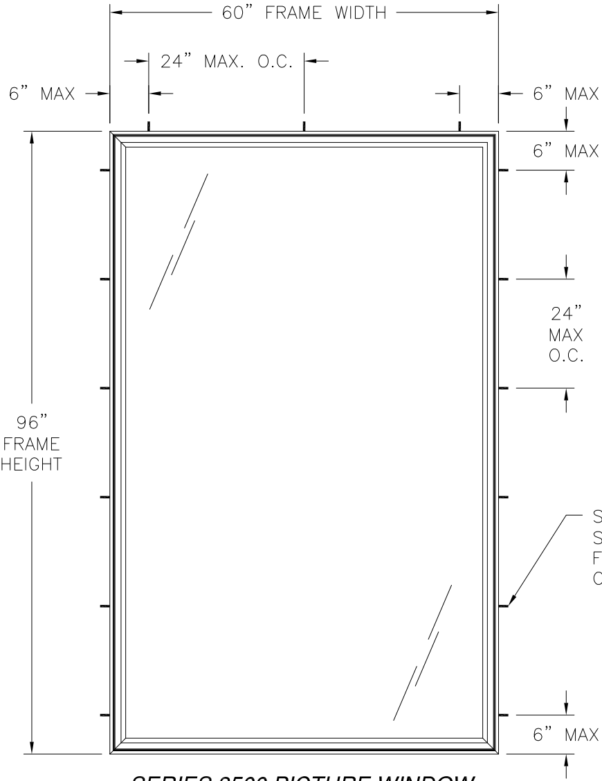
SERIES 3500 PICTURE WINDOW EXTERIOR VIEW FINLESS & FLANGE INSTALLATION
