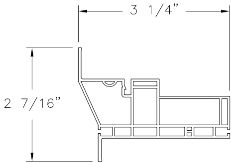
MAIN FRAME W/FLANGE EXTRUDED RIGID PVC (V-768)
