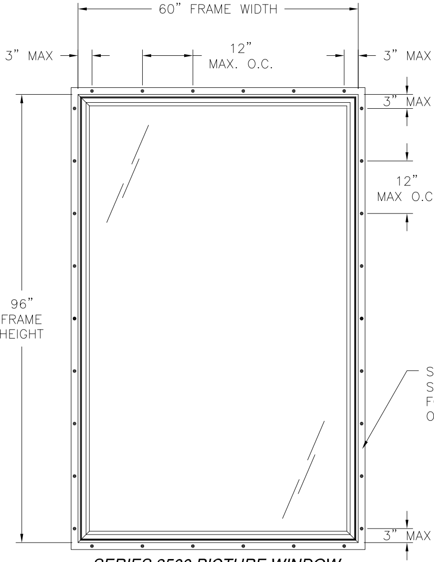
SERIES 3500 PICTURE WINDOW EXTERIOR VIEW FIN INSTALLATION
