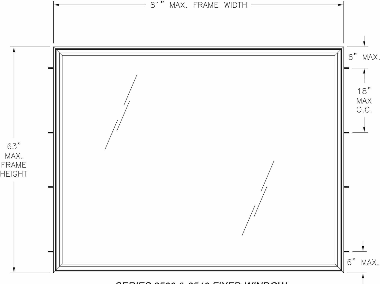
SERIES 3500 & 3540 FIXED WINDOW EXTERIOR VIEW FINLESS & FLANGE INSTALLATION
