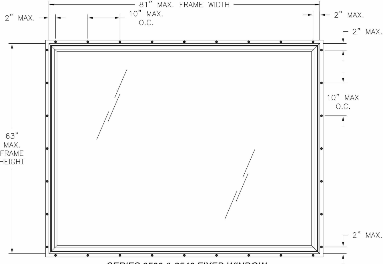
SERIES 3500 & 3540 FIXED WINDOW EXTERIOR VIEW FIN INSTALLATION
