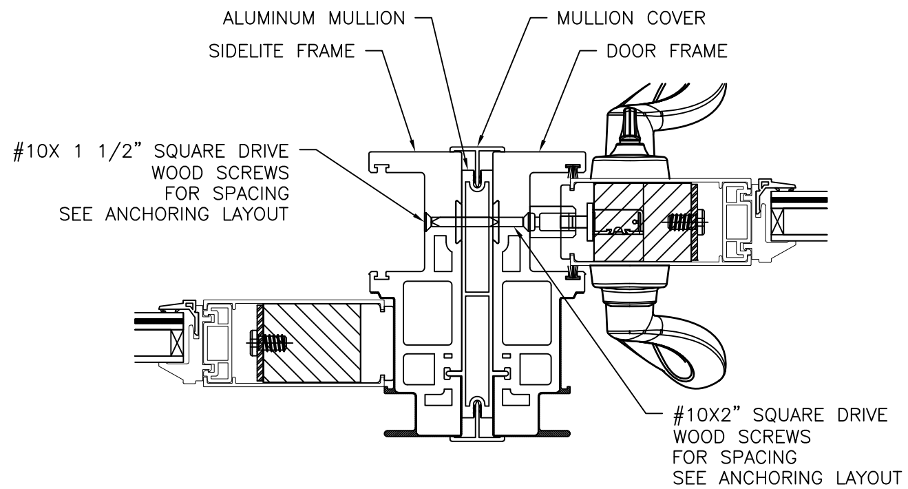
MULLION CONNECTION DETAIL
