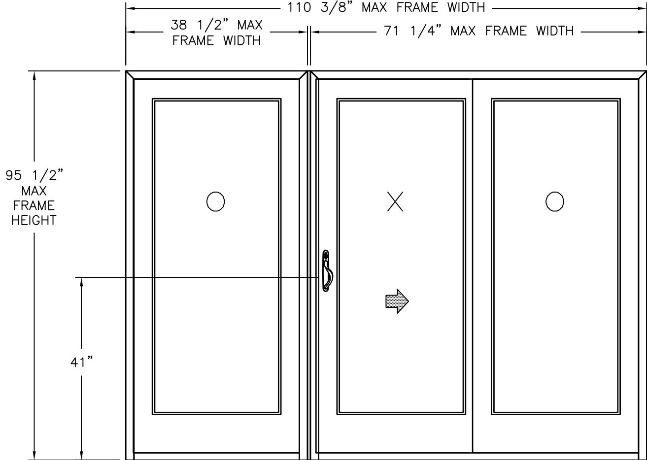
SERIES O/XO GLIDING PATIO DOOR EXTERIOR VIEW
